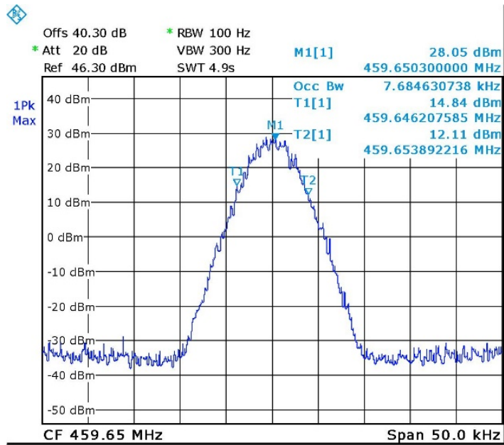
Figure 22. 99% Occupied BW, digital
