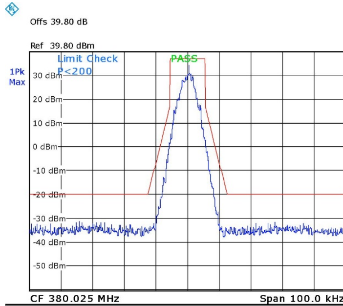
Figure 19. 380.025MHz, TDMA
