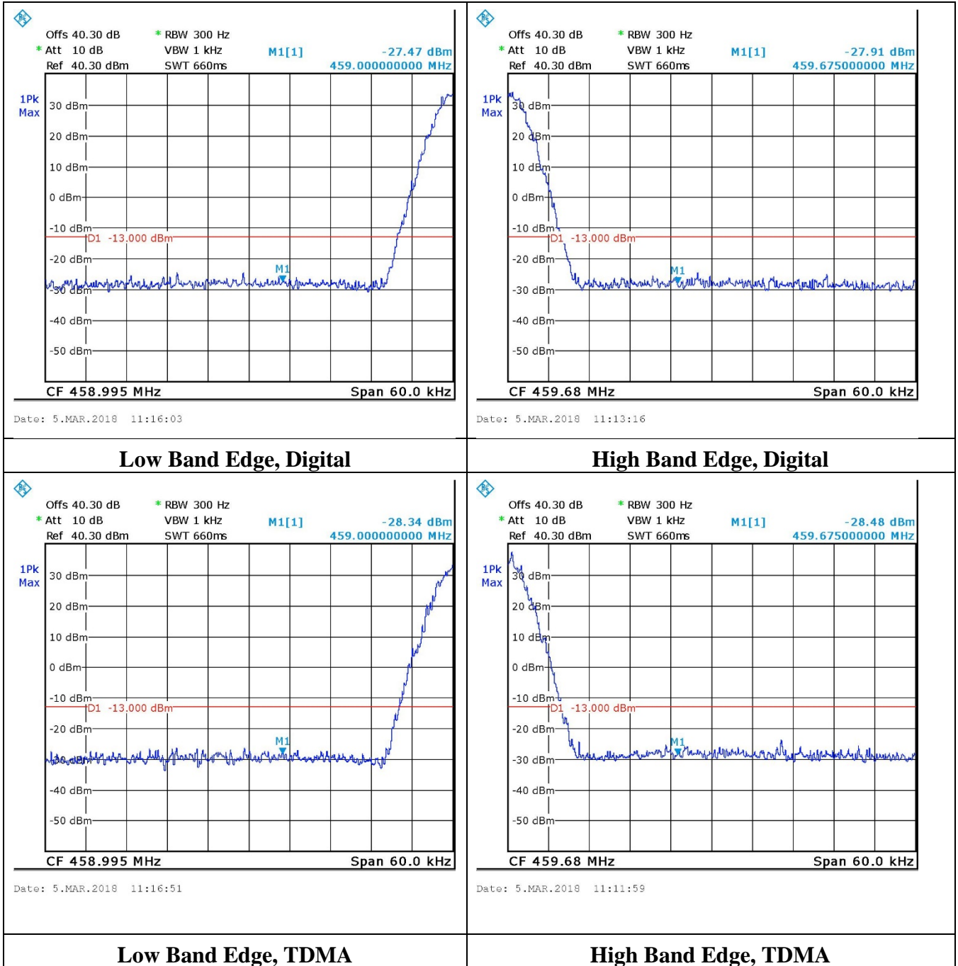
Figure 32 Band Edge Spectrum Results
