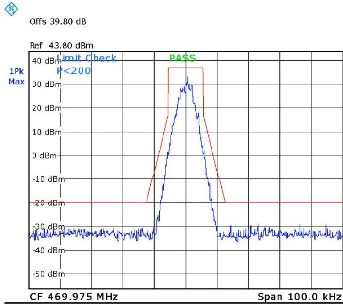
Figure 21. 469.975MHz, TDMA
