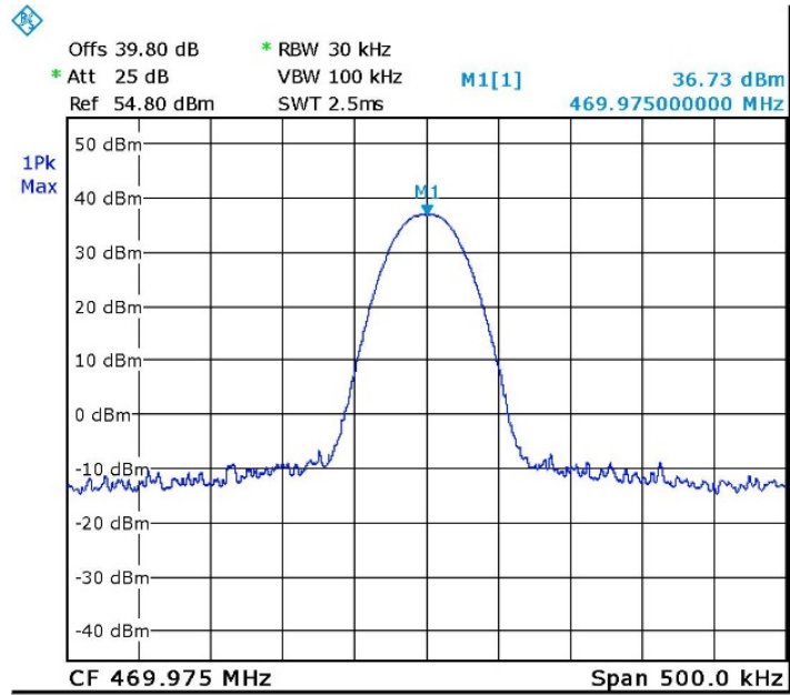
Figure 11. 469.975MHz, Digital
