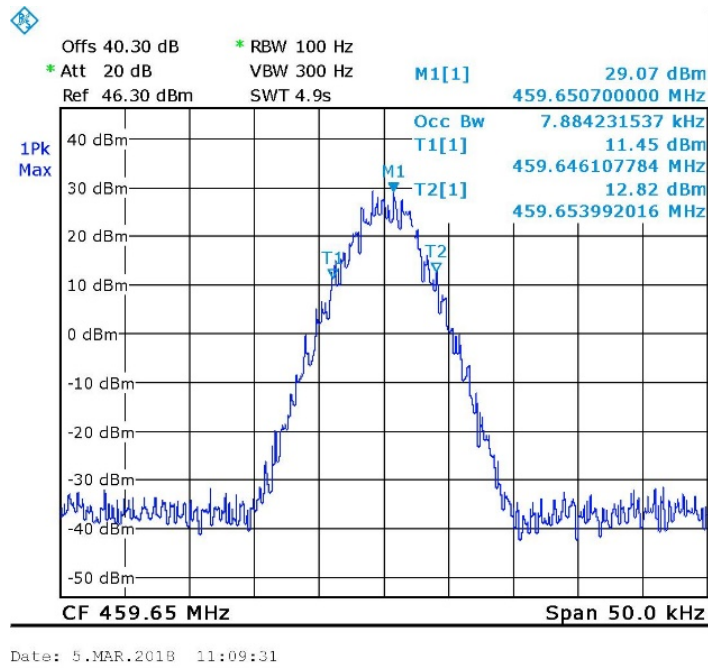
Figure 23. 99% Occupied BW, TDMA
