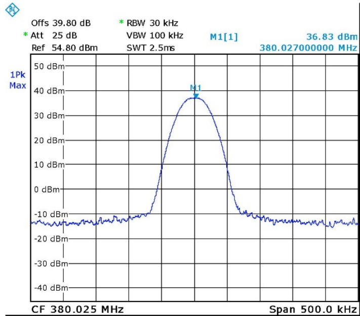
Figure 12. 380.025MHz, TDMA
