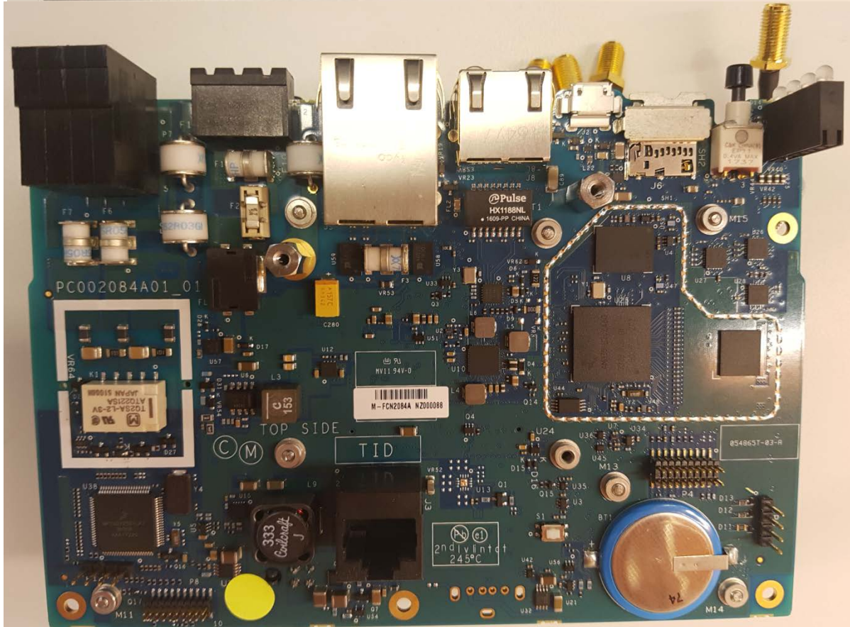
MC-EDGE CPU Board Top View Without Front Panel
