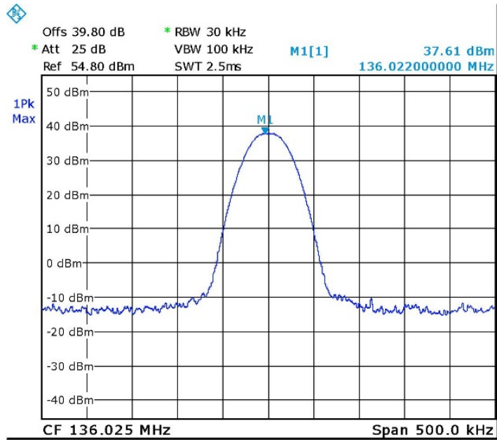
Figure 12. 136.025MHz, TDMA
