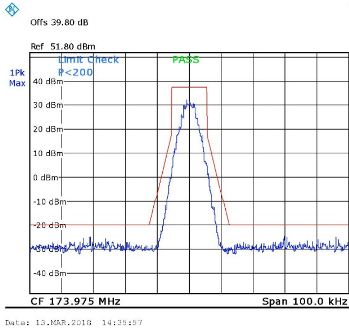
Figure 18. 173.975MHz, Digital
