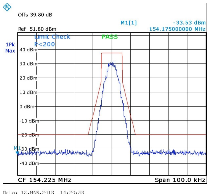
Figure 17. 154.225MHz, Digital
