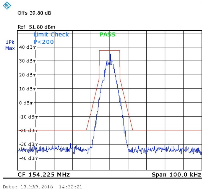
Figure 20. 154.225MHz, TDMA
