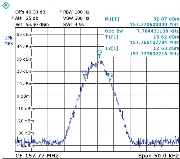
Figure 22. 99% OBW, Digital
