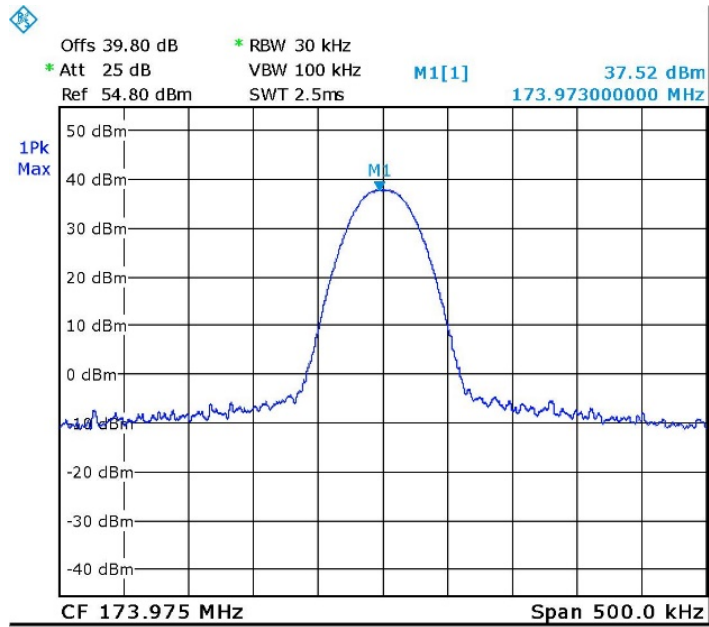
Figure 11. 173.975MHz, Digital
