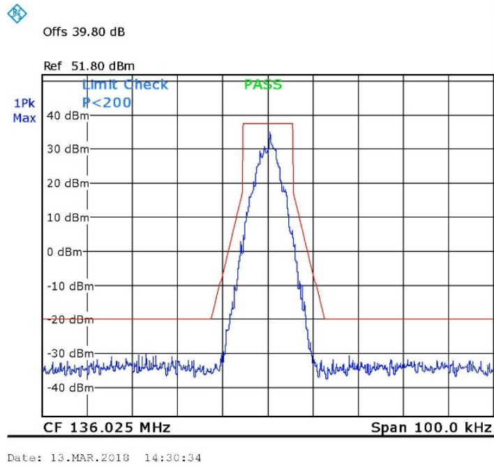
Figure 19. 136.025MHz, TDMA
