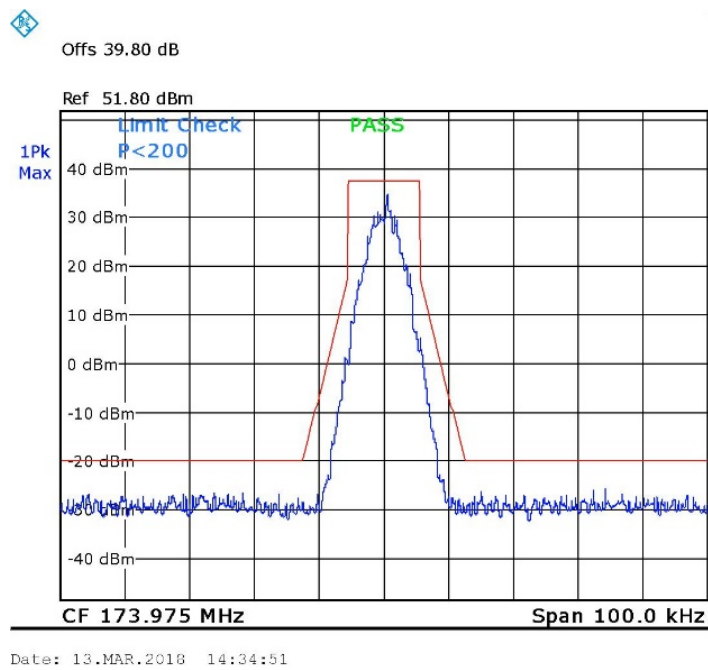
Figure 21. 173.975MHz, TDMA
