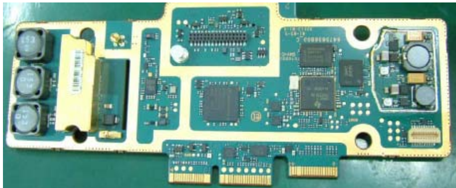
Controller board without Shields (Bottom)
