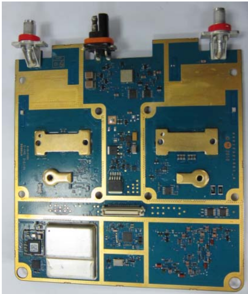
RF board with Shields (Bottom)
