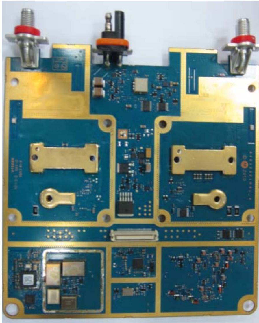
RF board without Shields (Bottom)
