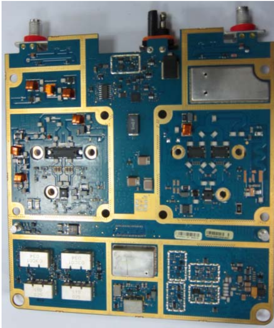
RF board with Shields (Top)
