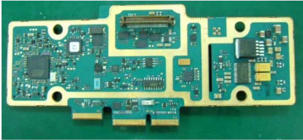
Controller board with Shields (Top)
