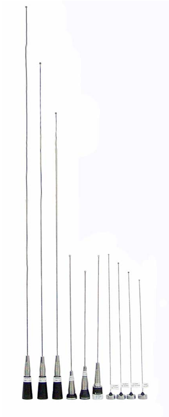
Antenna kit numbers, from left to right; RAD4010ARB (136MHz), RAD4010ARB (150MHz), RAD4010ARB (174MHz), HAD4016A, HAD4017A, HAD4021A, HAD4006A, HAD4007A, HAD4008A, HAD4009A
