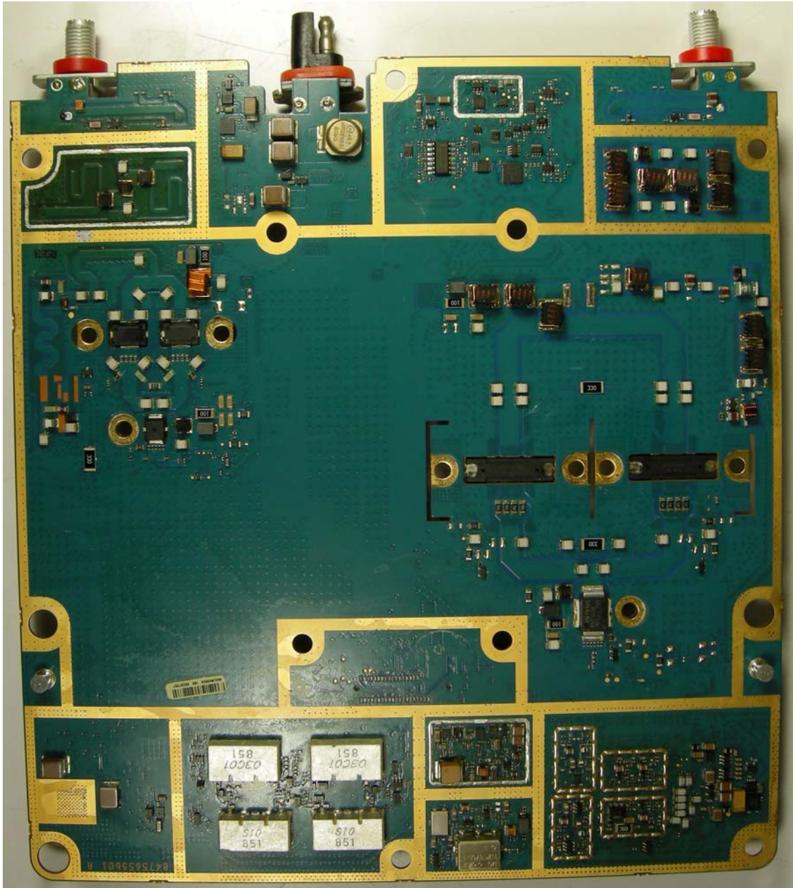
RF BOARD, LESS SHIELD (TOP VIEW)
