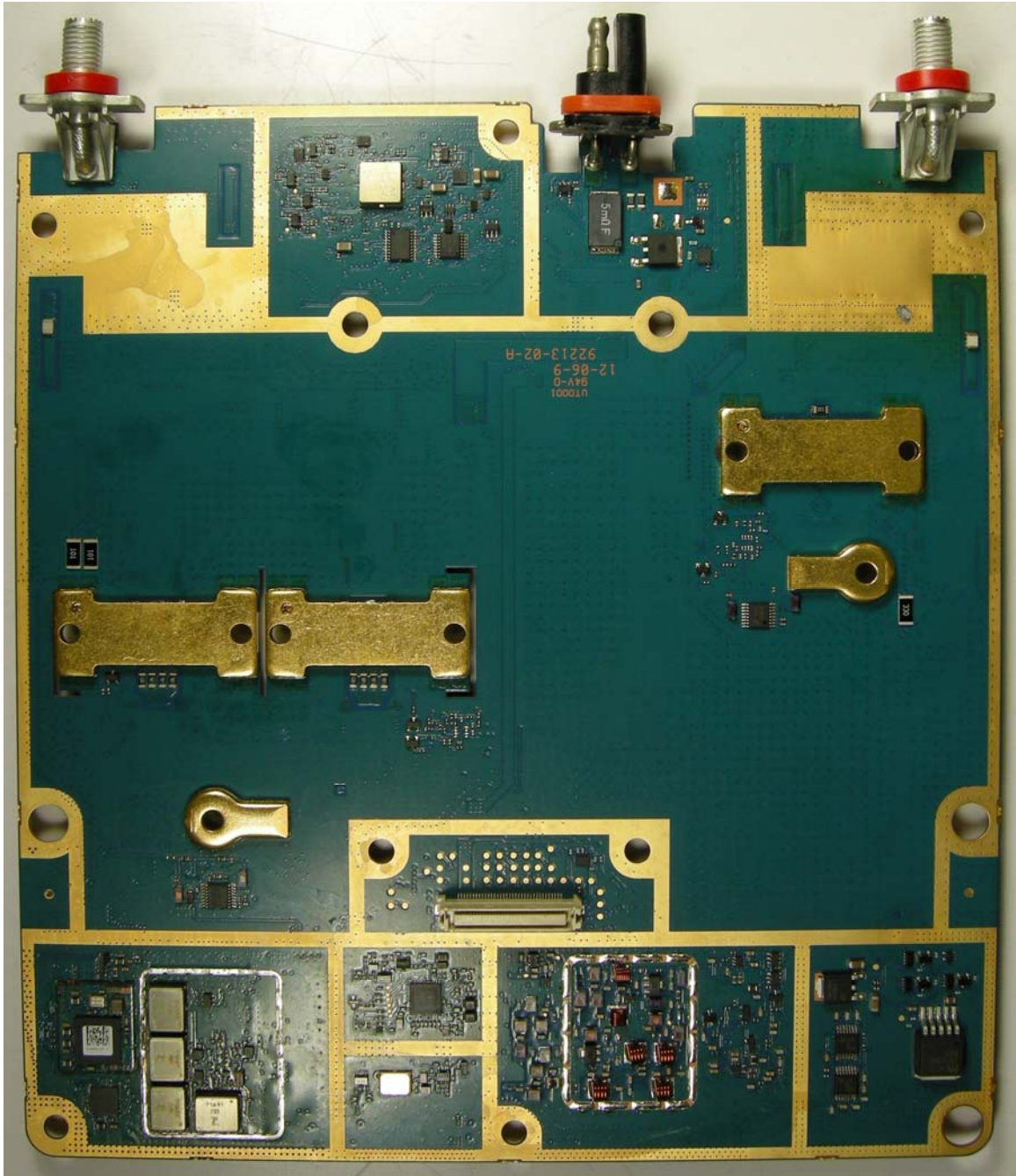
RF BOARD, LESS SHIELD (BOTTOM VIEW)
