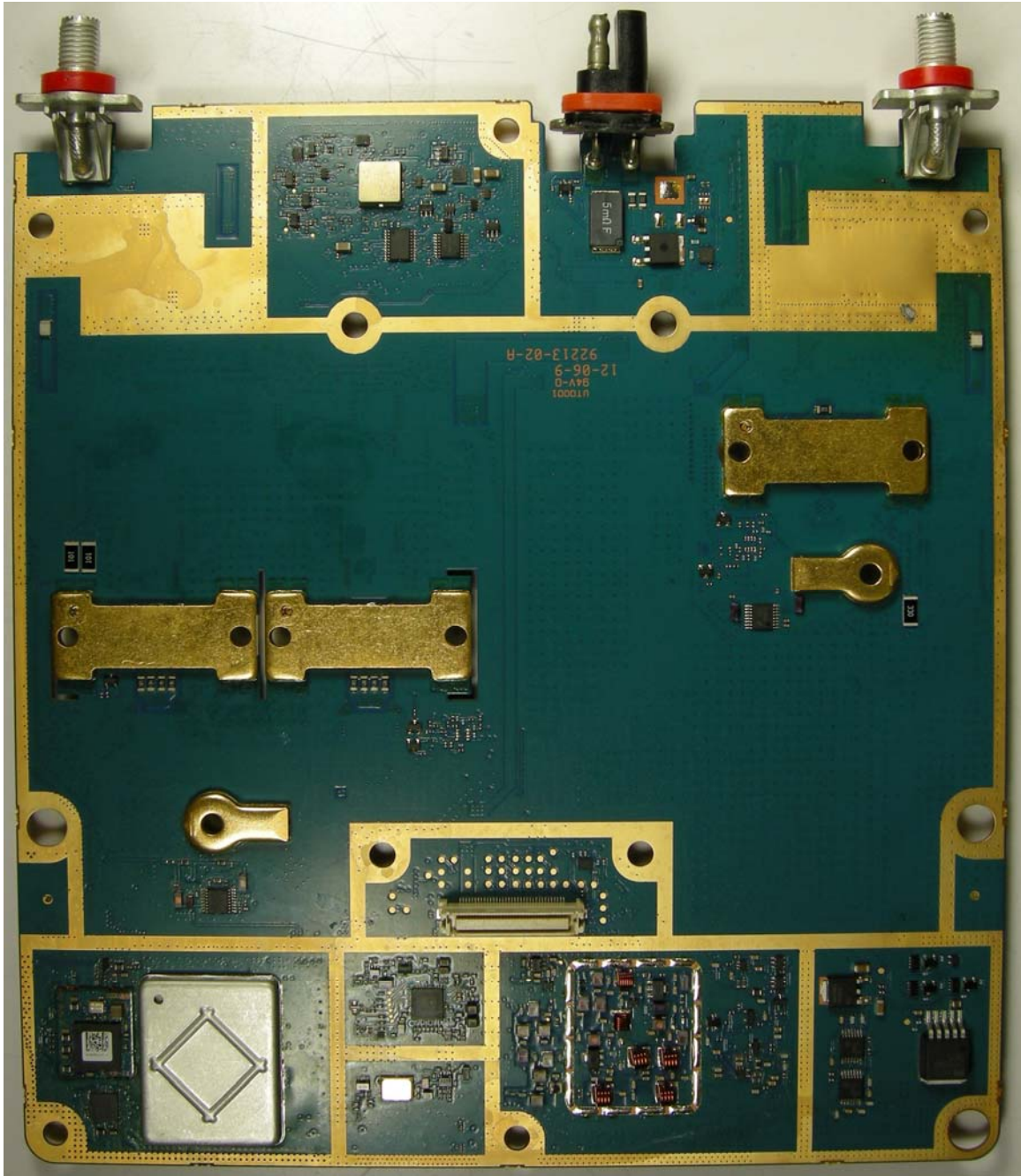
RF BOARD (BOTTOM VIEW)
