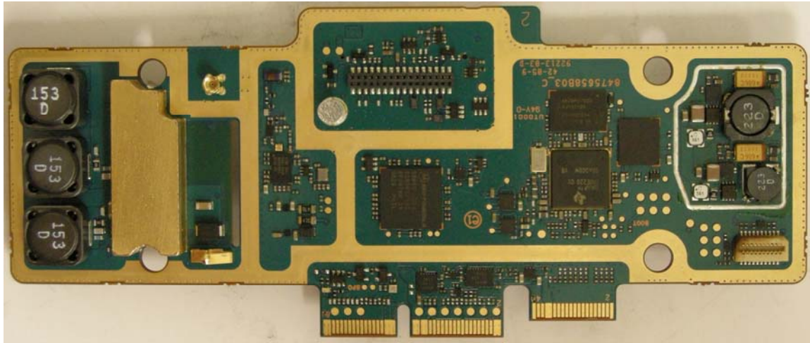
CONTROLLER BOARD, LESS SHIELD (BOTTOM VIEW)
