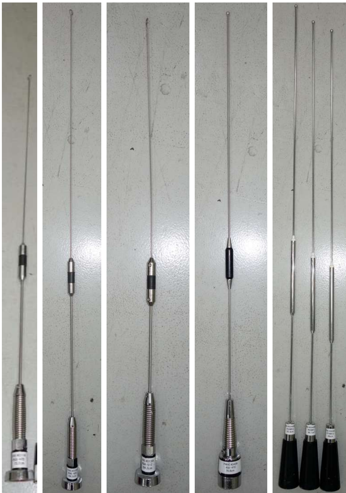
UHF2 Antenna kit numbers, from left to right HAE4011A, HAE4012A, HAE4013A, PMAE4043A, *RAE4004ARB (3pcs)
