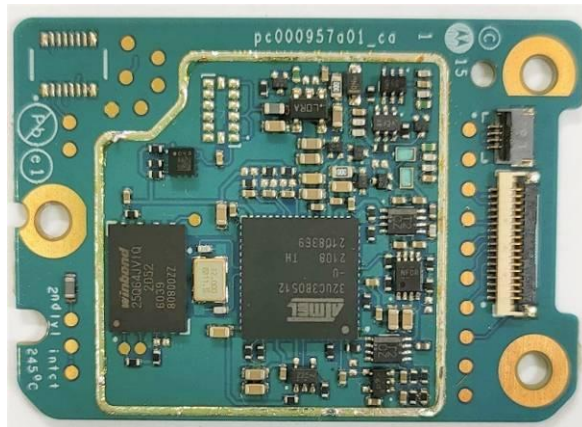
GOB_Rev A board without shield (Bottom)
