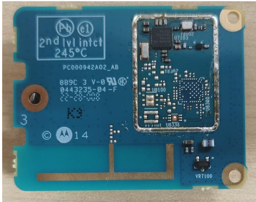
Expansion board without shield (Bottom)
