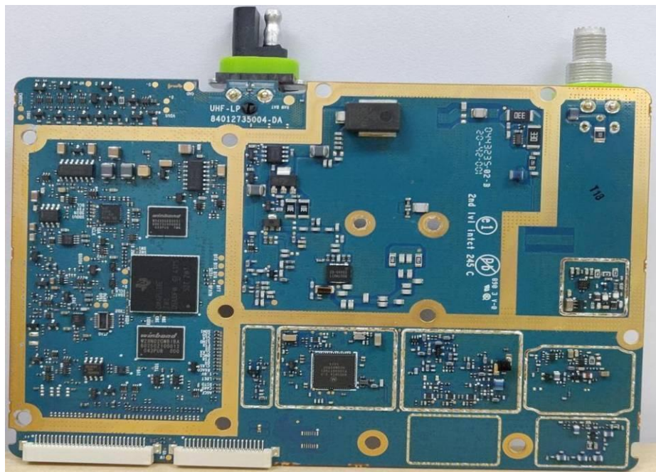
RF board without Shields (Bottom)
