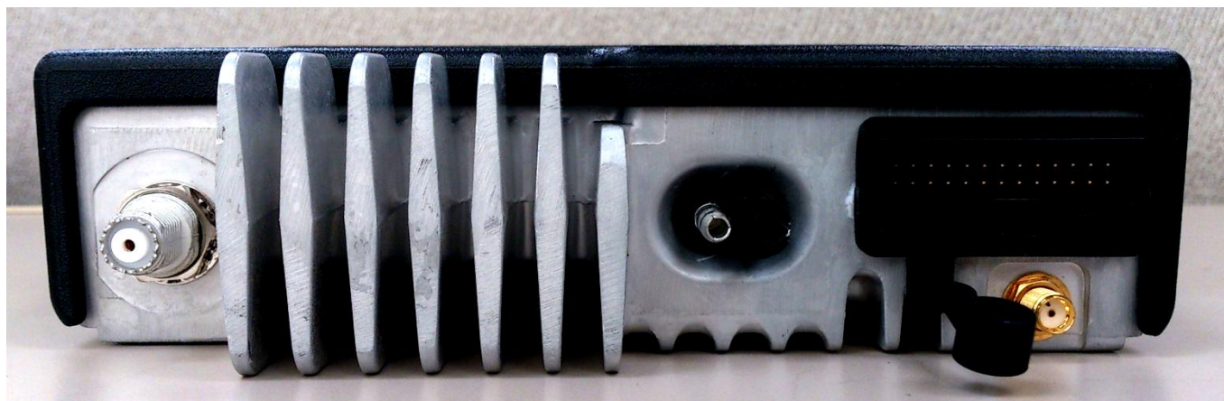
Back View (same for XPR 5550e Color Display and XPR 5350e Numeric Display)
