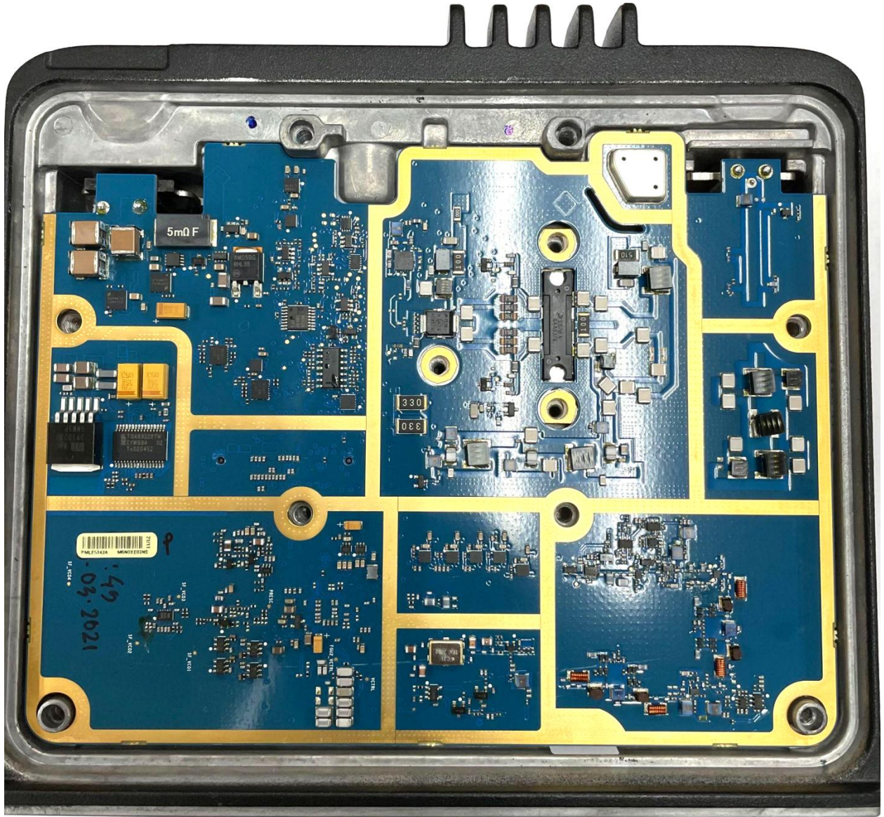
Exhibit 9G: Radio Assembly – RF Board (Top View)
