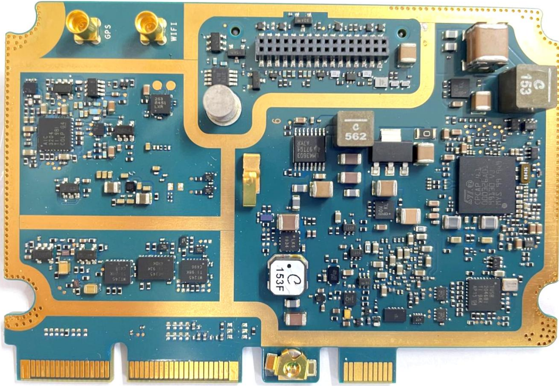
Exhibit 9F: Controller Board (Bottom)
