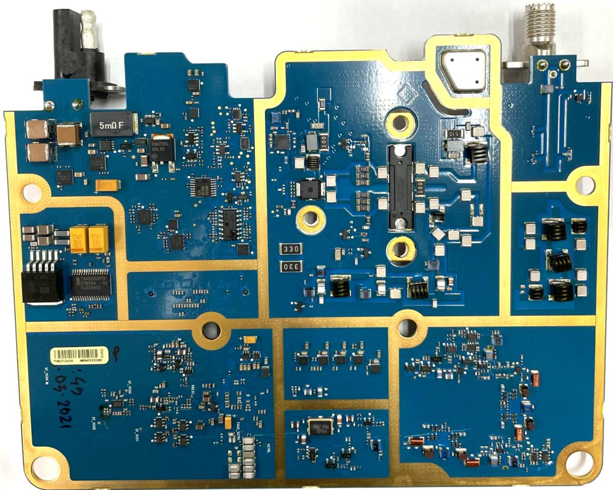
Exhibit 9A: RF Board with Shields (Top)
