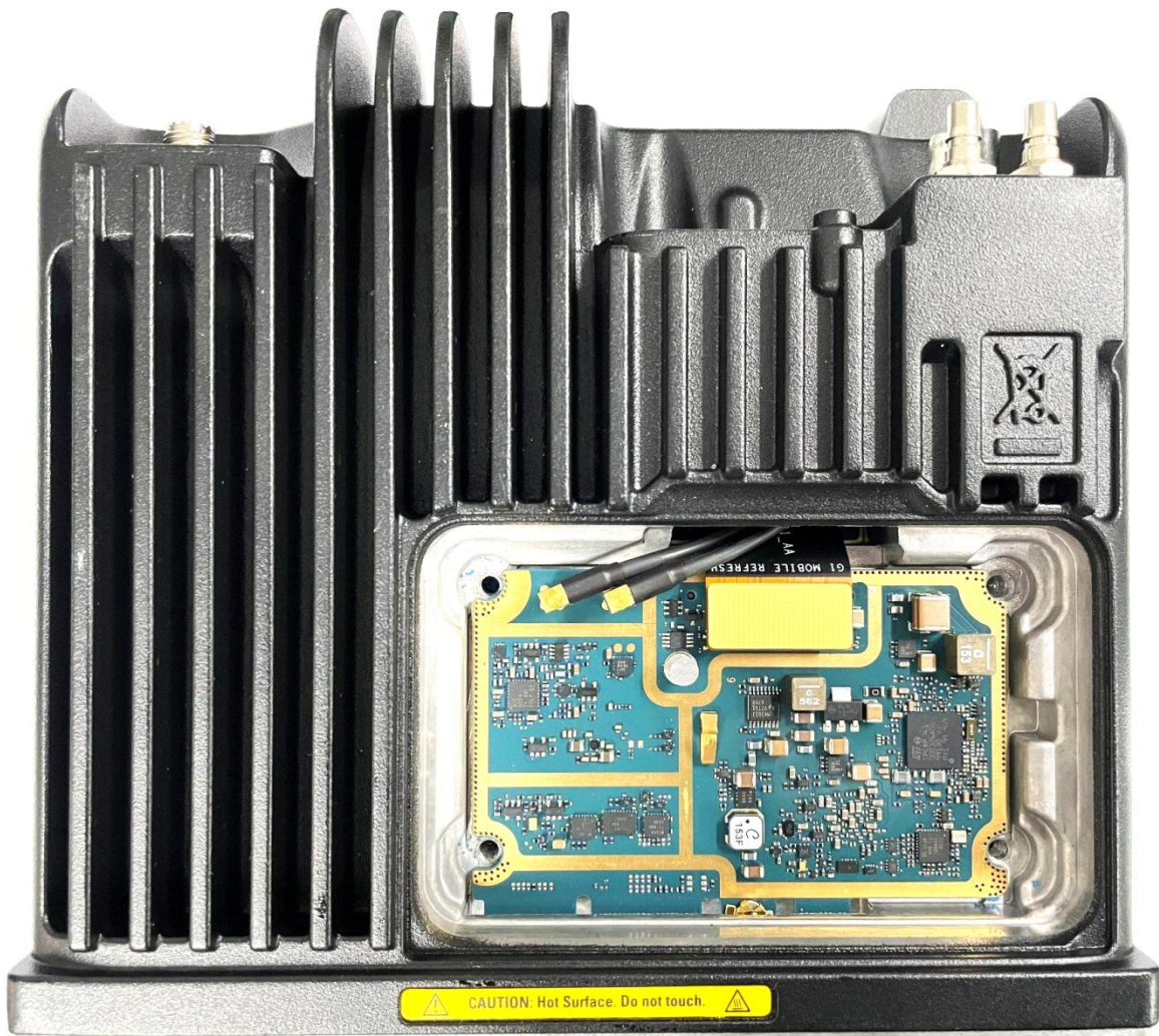
Exhibit 9H: Radio Assembly – Controller Board (Bottom View)
