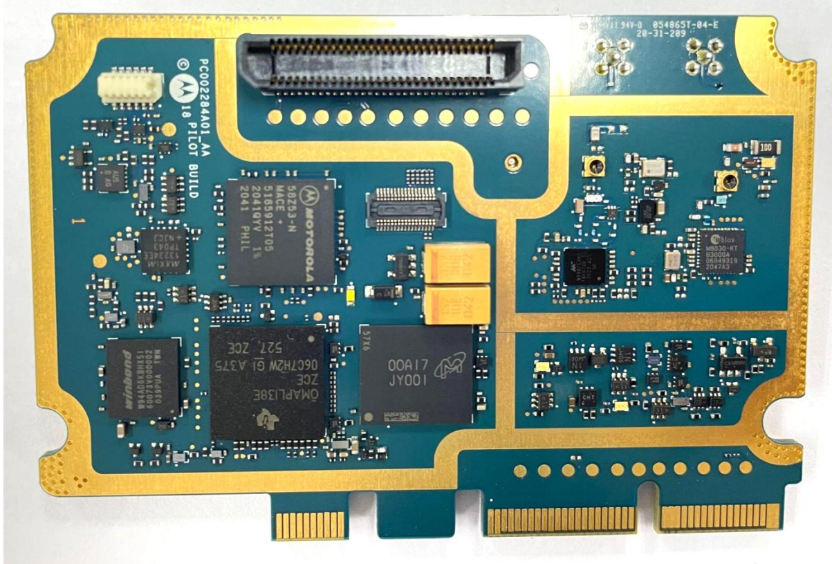
Exhibit 9E: Controller Board (Top)
