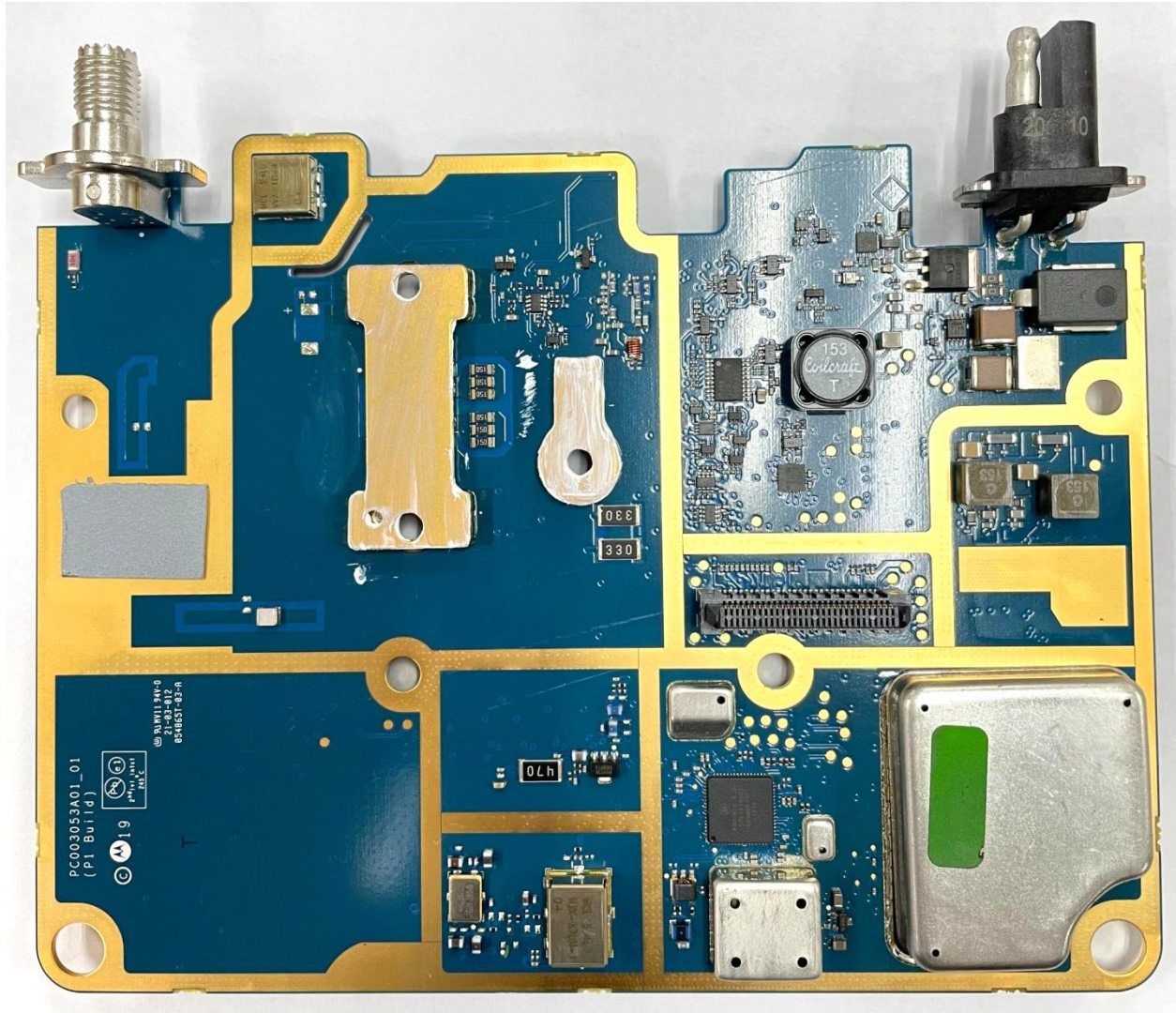
Exhibit 9C: RF Board with Shields (Bottom)
