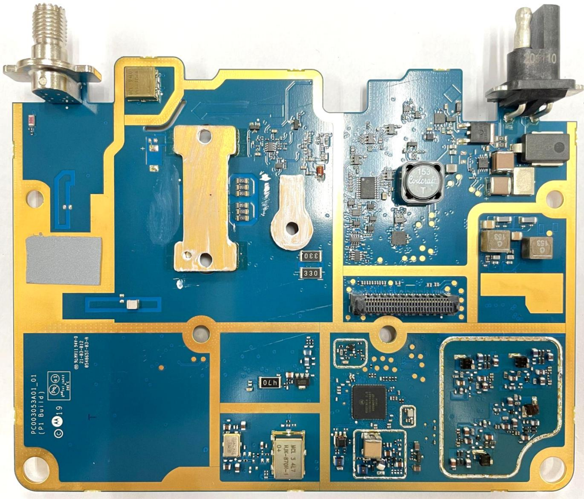
Exhibit 9D: RF Board without Shields (Bottom)
