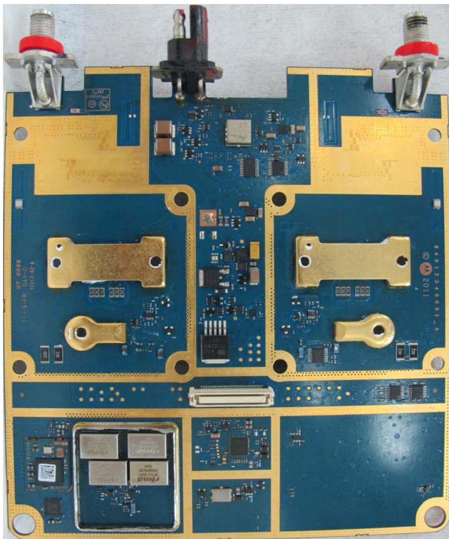
RF board without Shields (Bottom)
