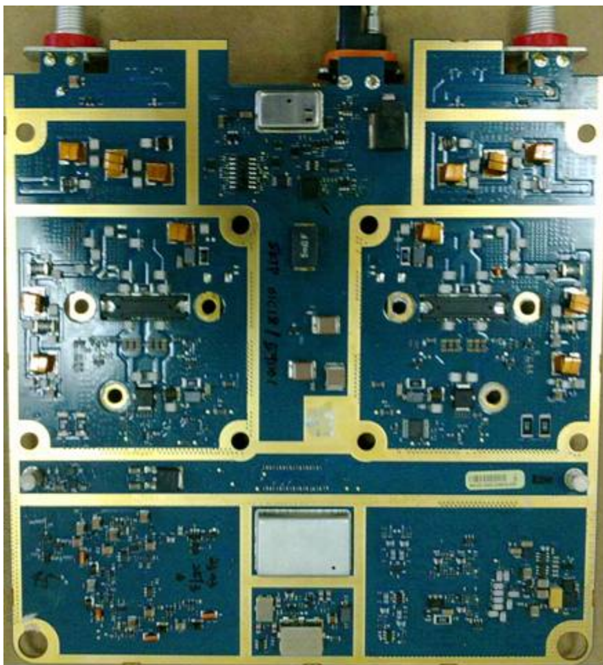
RF board with Shields (Top)
