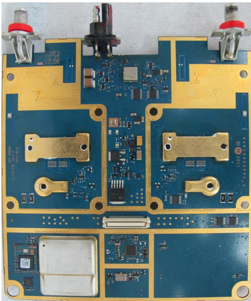
RF board with Shields (Bottom)
