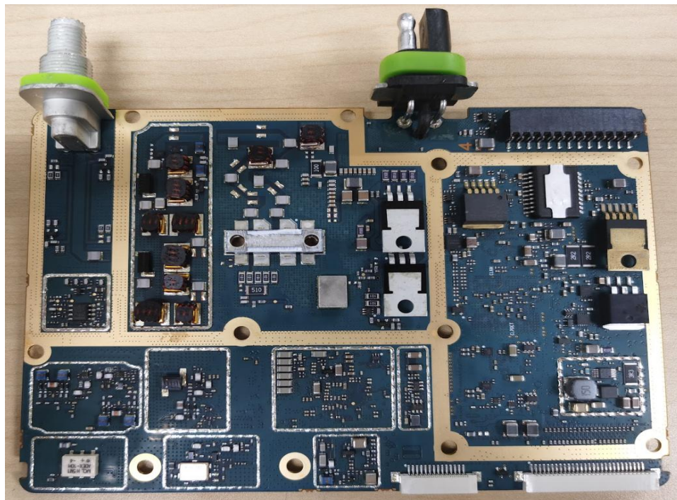
RF board without Shields (Top)
