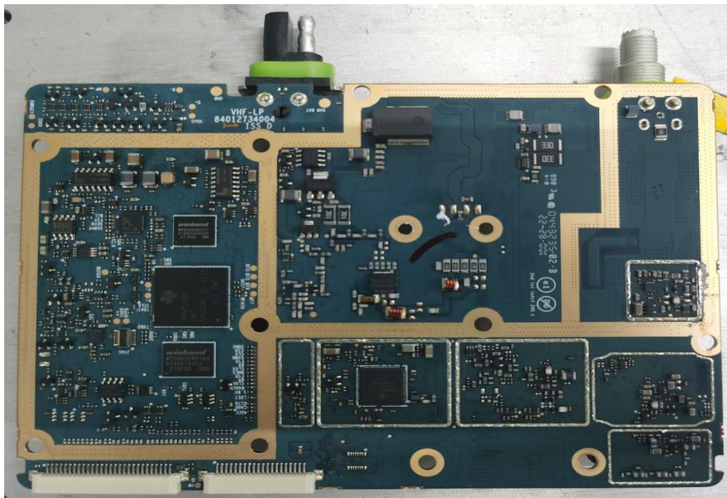
RF board without Shields (Bottom)
