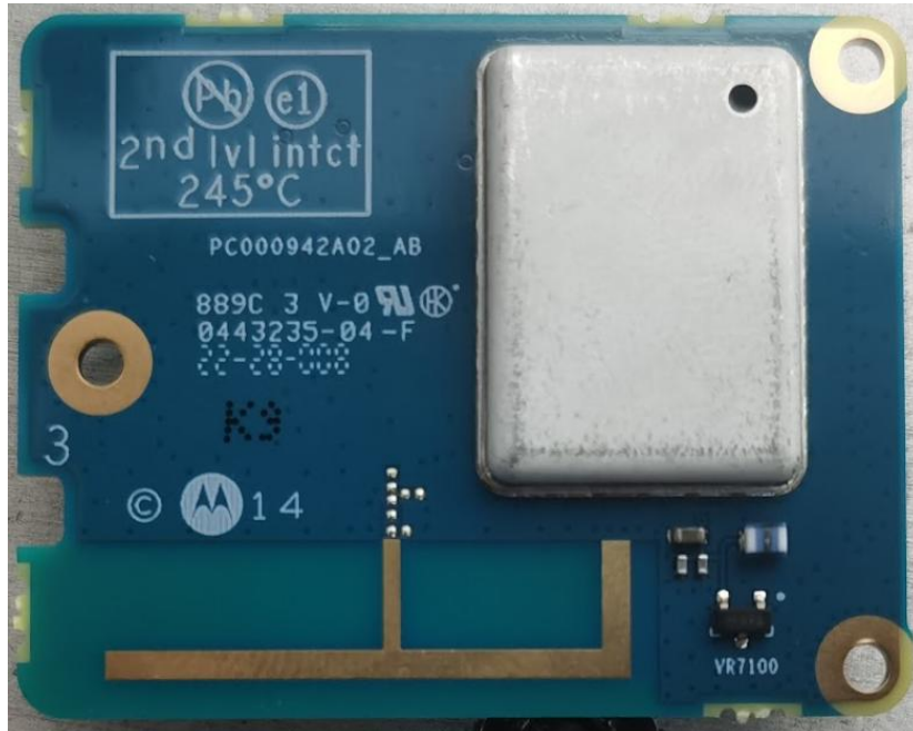
GNSS Expansion board with Shields (Bottom)
