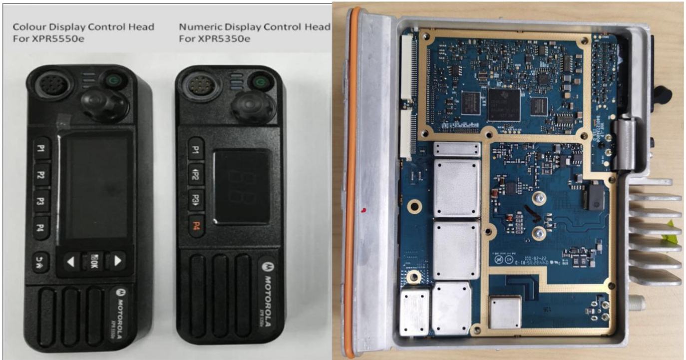
Chassis and control heads (Top)
