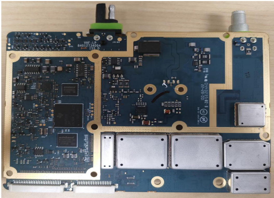
RF board with Shields (Bottom)
