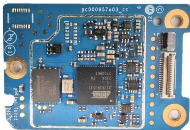
GOB_Rev C board without shield (Bottom)
