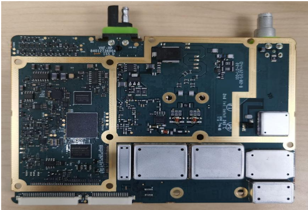
RF board with Shields (Bottom)
