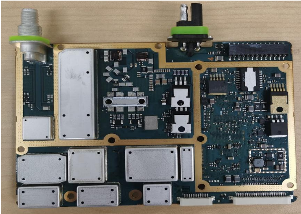
RF board with Shields (Top)
