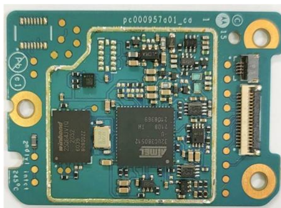
GOB_Rev A board without shield (Bottom)
