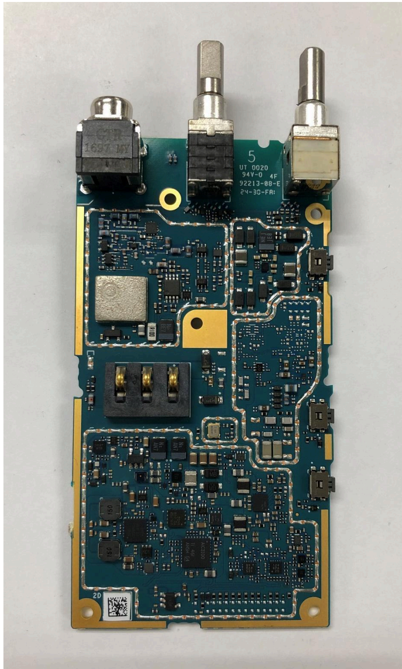
RF board without Shields (Bottom) of LKP Model
