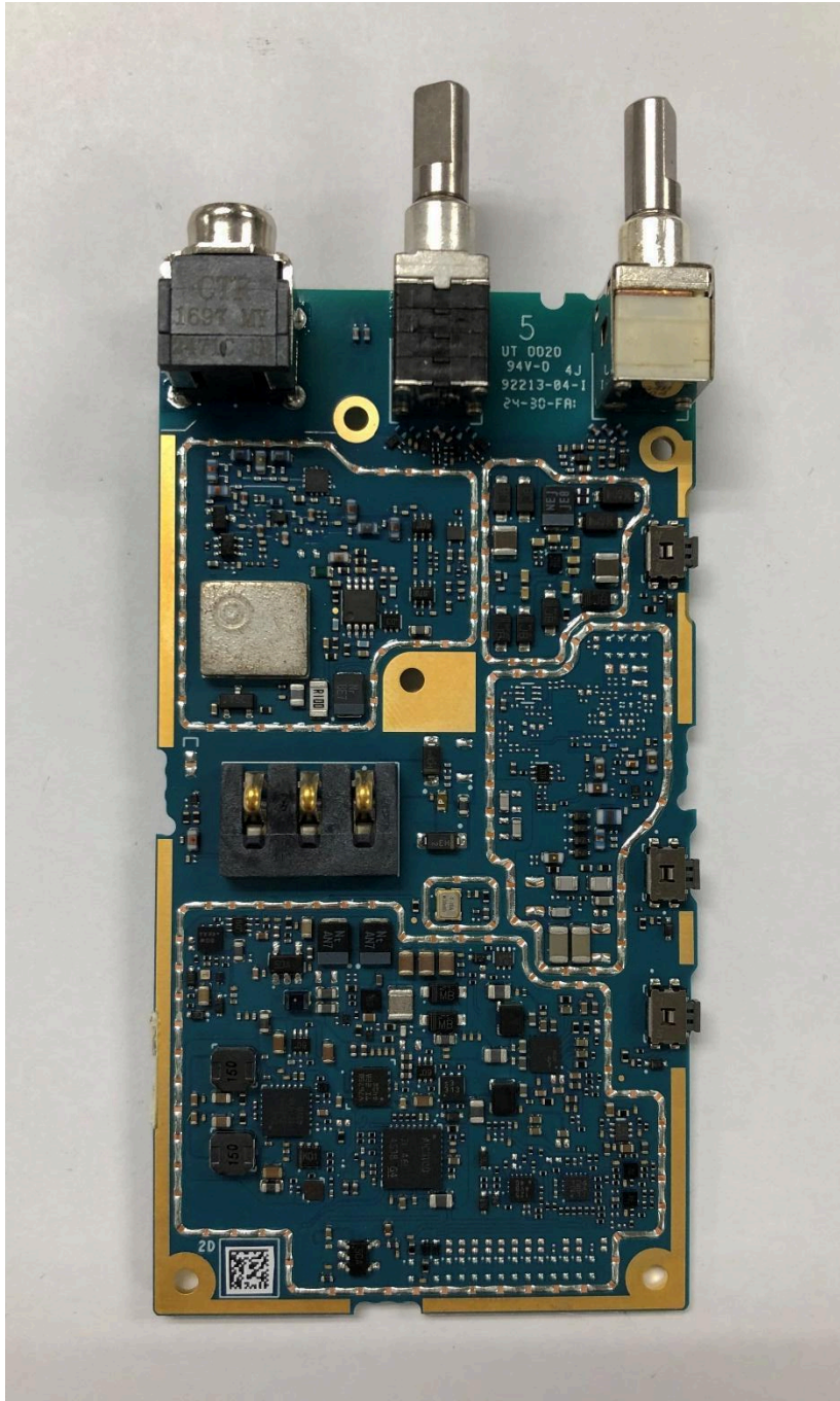
RF board without Shields (Bottom) of NKP Model
