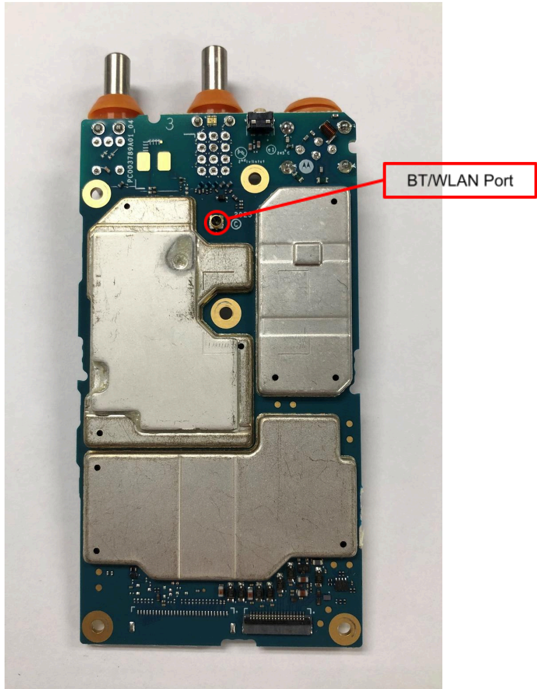
RF board with Shields (Top) of NKP Model
