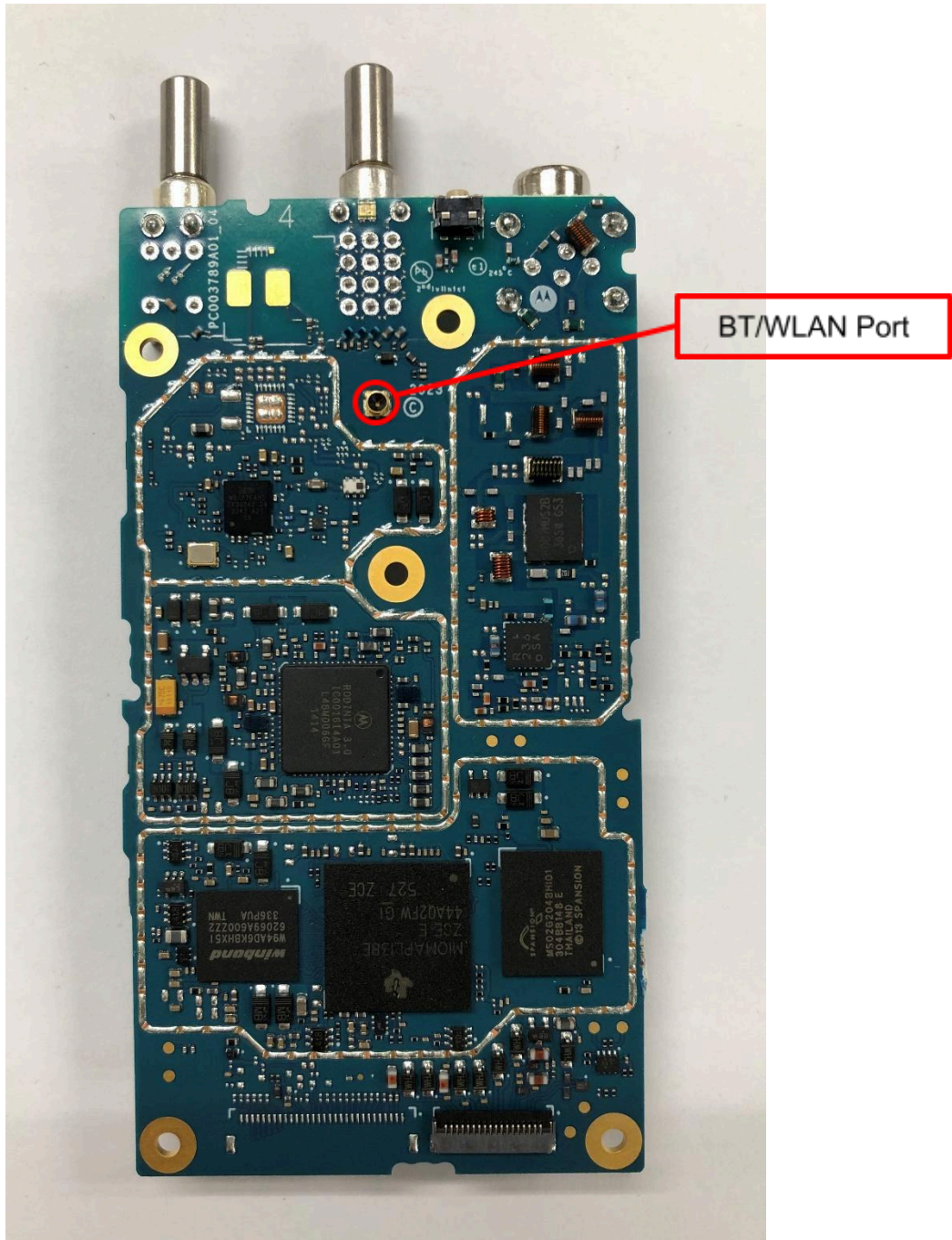
RF board without Shields (Top) of NKP Model
