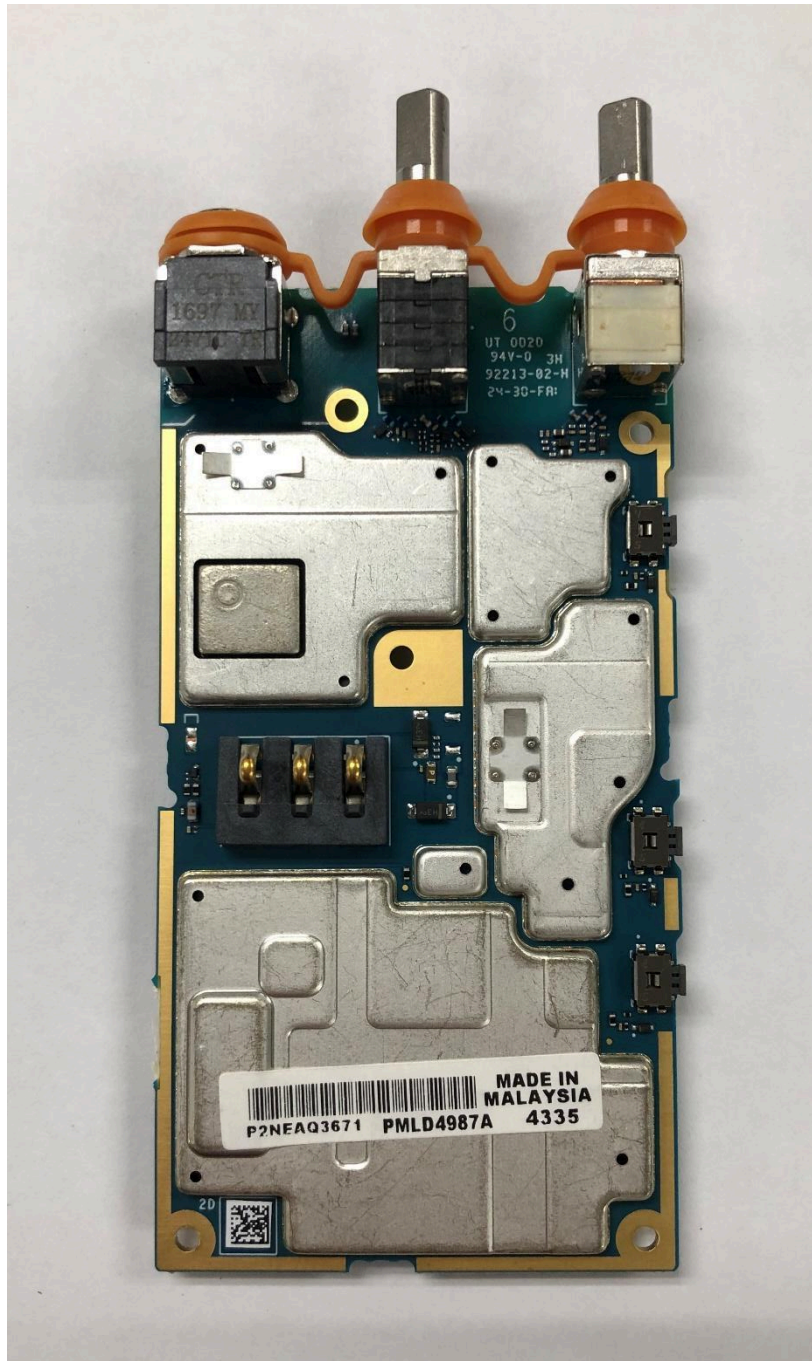
RF board with Shields (Bottom) of NKP Model
