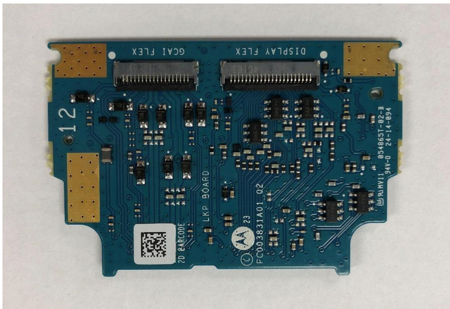
Keypad Board (Bottom) of LKP Model
