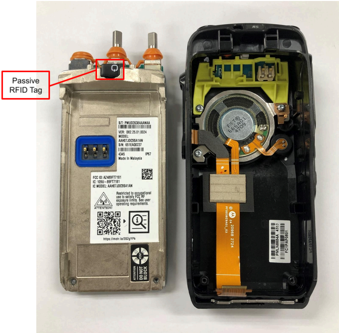
Chassis and Housing (Back Side) of NKP Model
