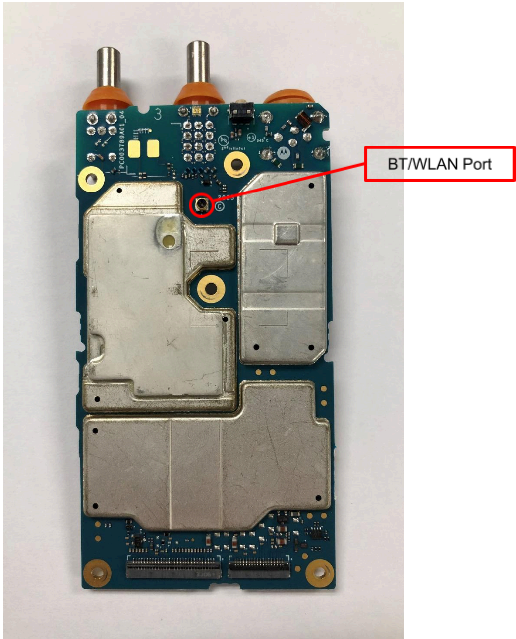
RF board with Shields (Top) of LKP Model
