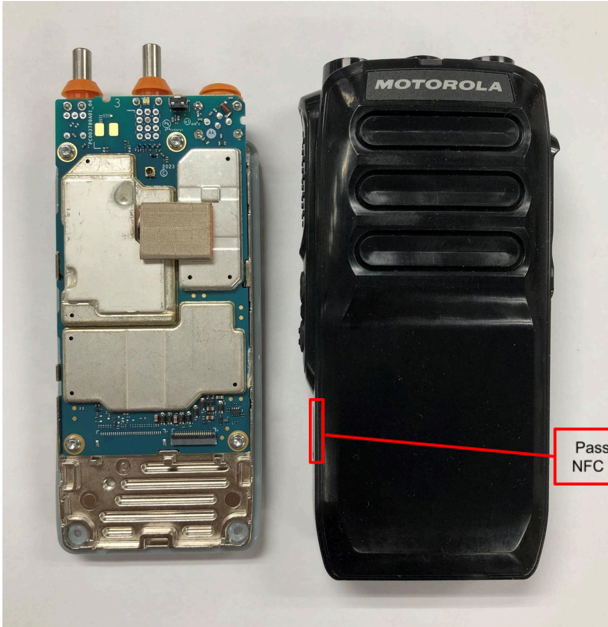
RF boards with chassis and housing for (Front Side) of NKP Model
