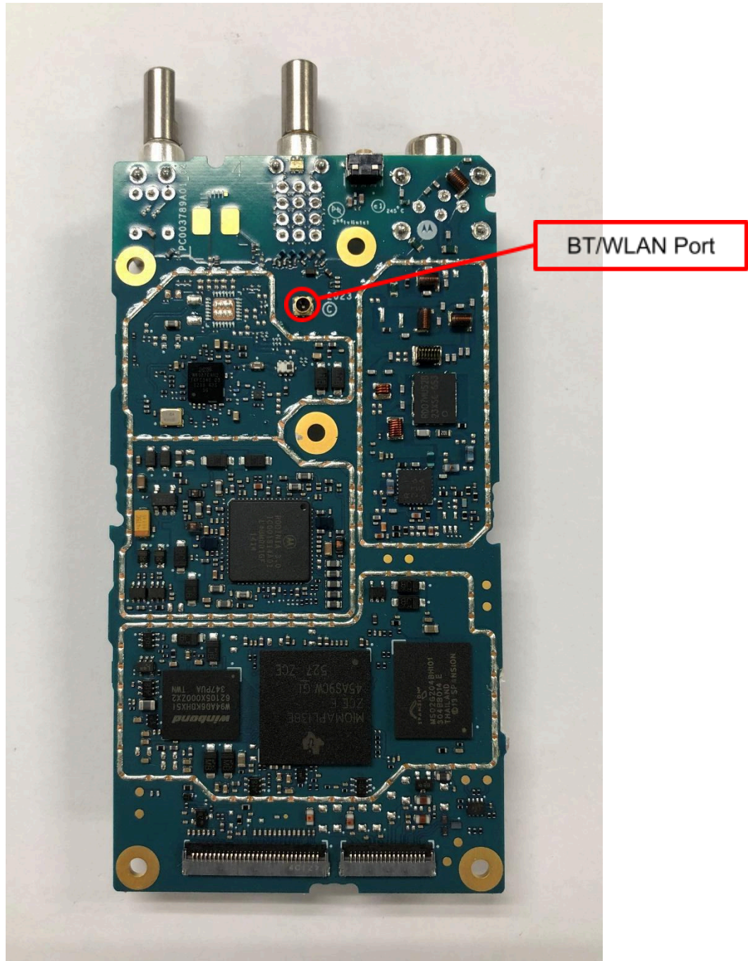
RF board without Shields (Top) of LKP Model
