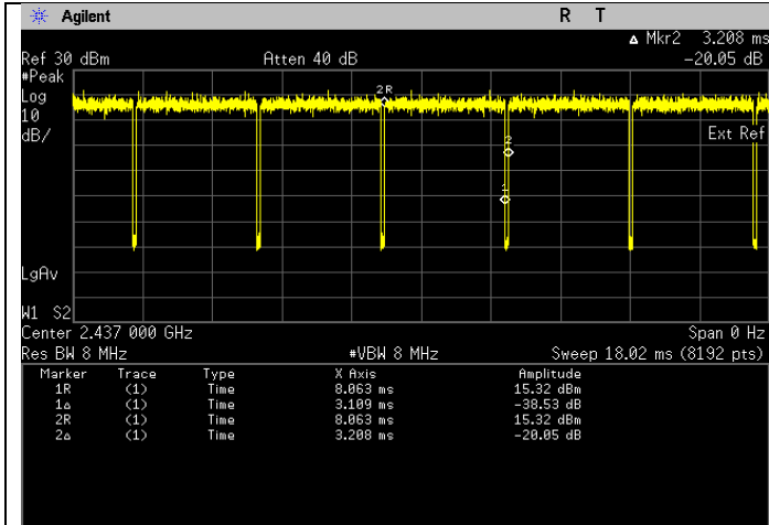
Duty Cycle
