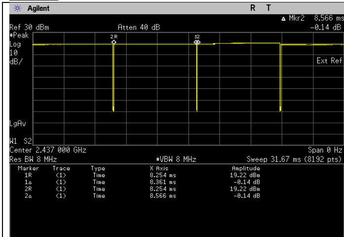
Duty Cycle
