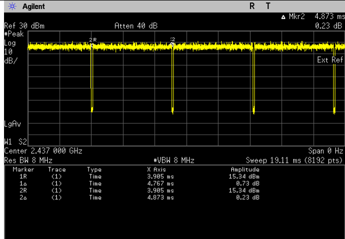
Duty Cycle
