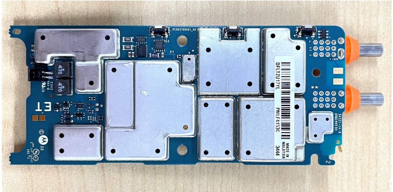
RF Board with Shields (Top), MTP3500/MTP3550 800 MHz series
