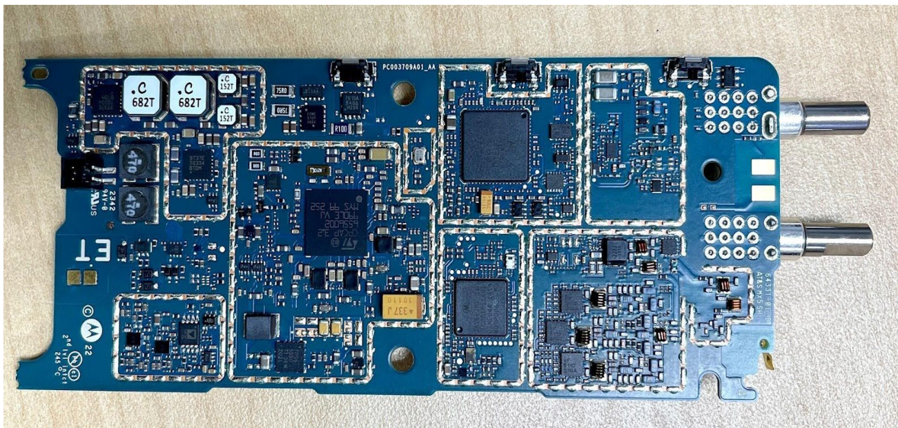
RF Board without Shields (Top), MTP3500/MTP3550 800 MHz series
