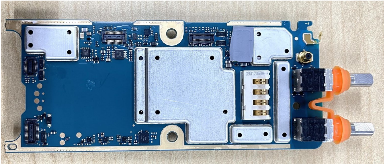
RF Board with Shields (Bottom), MTP3500/MTP3550 800 MHz series
