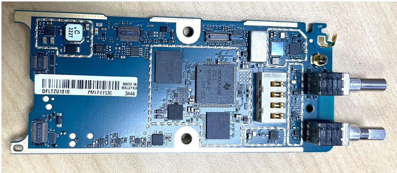
RF Board without Shields (Bottom), MTP3500/MTP3550 800 MHz series
