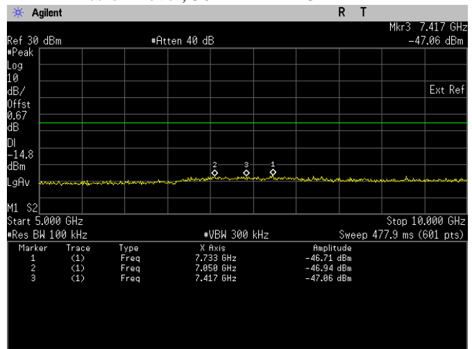
Conducted Emissions. Bluetooth LE, Frequency 2478 MHz Emission Level, 5 GHz -> 10 GHz
