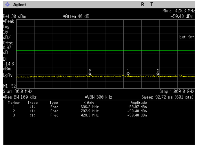
Conducted Emissions. Bluetooth LE, Frequency 2478 MHz Emission Level, 30 MHz -> 1 GHz
