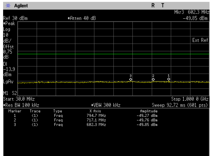
Conducted Emissions. Bluetooth LE, Frequency 2404 MHz Emission Level, 30 MHz -> 1 GHz
