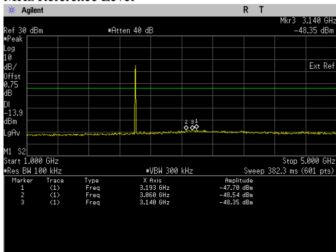
Conducted Emissions. Bluetooth LE, Frequency 2404 MHz Emission Level, 1 GHz -> 5 GHz
