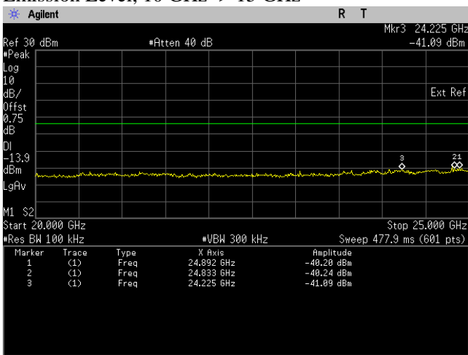
Conducted Emissions. Bluetooth LE, Frequency 2404 MHz Emission Level, 20 GHz -> 25 GHz
