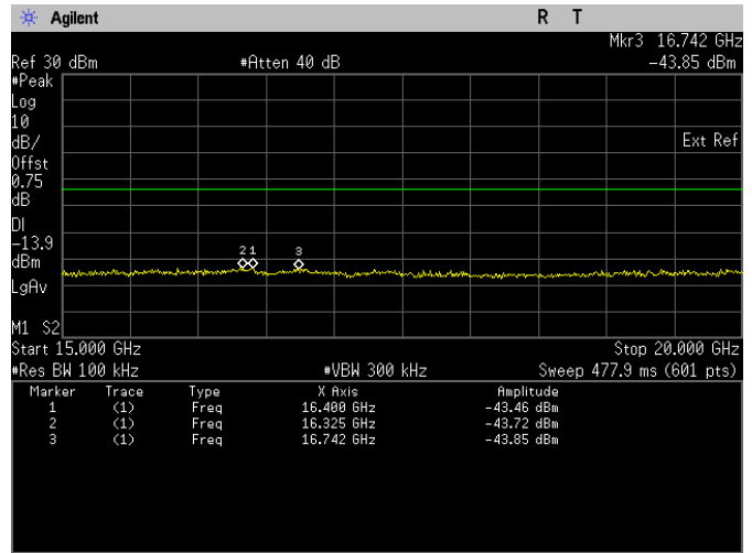
Conducted Emissions. Bluetooth LE, Frequency 2404 MHz Emission Level, 15 GHz -> 20 GHz
