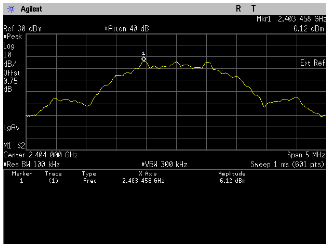
Conducted Emissions. Bluetooth LE, Frequency 2404 MHz Reference Level
