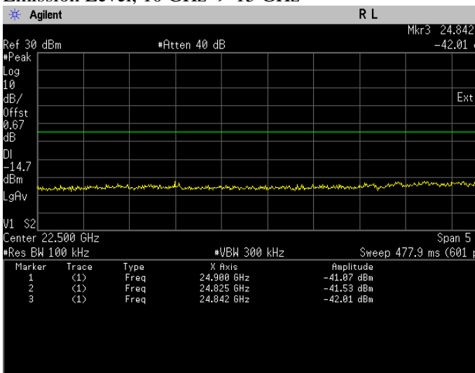
Conducted Emissions. Bluetooth LE, Frequency 2480 MHz Emission Level, 20 GHz -> 25 GHz
