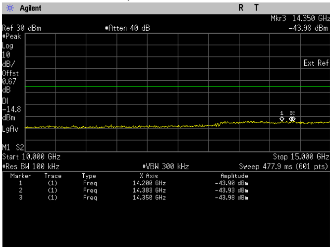
Conducted Emissions. Bluetooth LE, Frequency 2478 MHz Emission Level, 10 GHz -> 15 GHz
