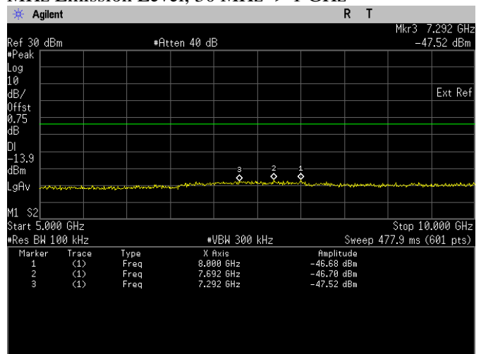
Conducted Emissions. Bluetooth LE, Frequency 2404 MHz Emission Level, 5 GHz -> 10 GHz
