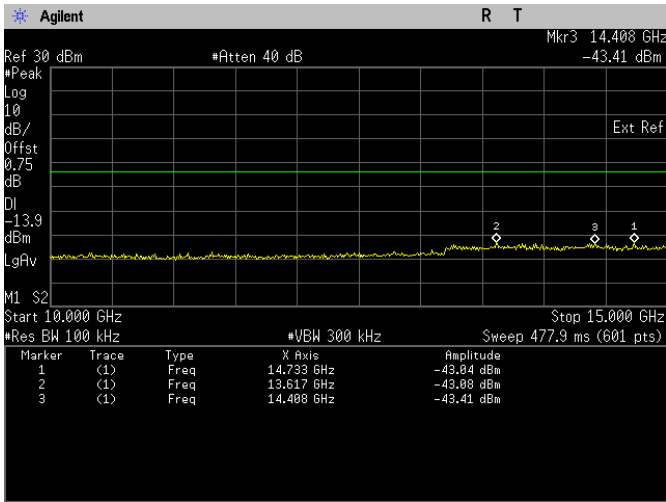
Conducted Emissions. Bluetooth LE, Frequency 2404 Emission Level, 10 GHz -> 15 GHz
