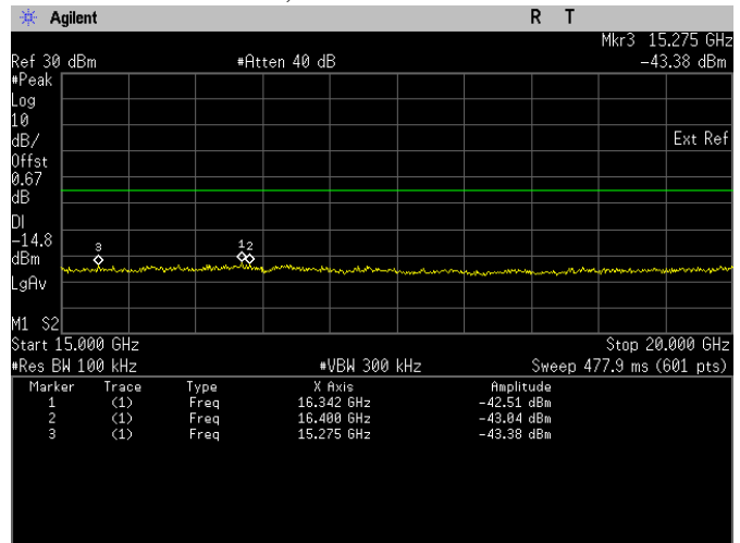
Conducted Emissions. Bluetooth LE, Frequency 2478 MHz Emission Level, 15 GHz -> 20 GHz
