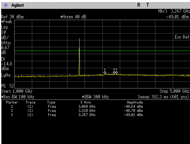
Conducted Emissions. Bluetooth LE, Frequency 2478 MHz Emission Level, 1 GHz -> 5 GHz
