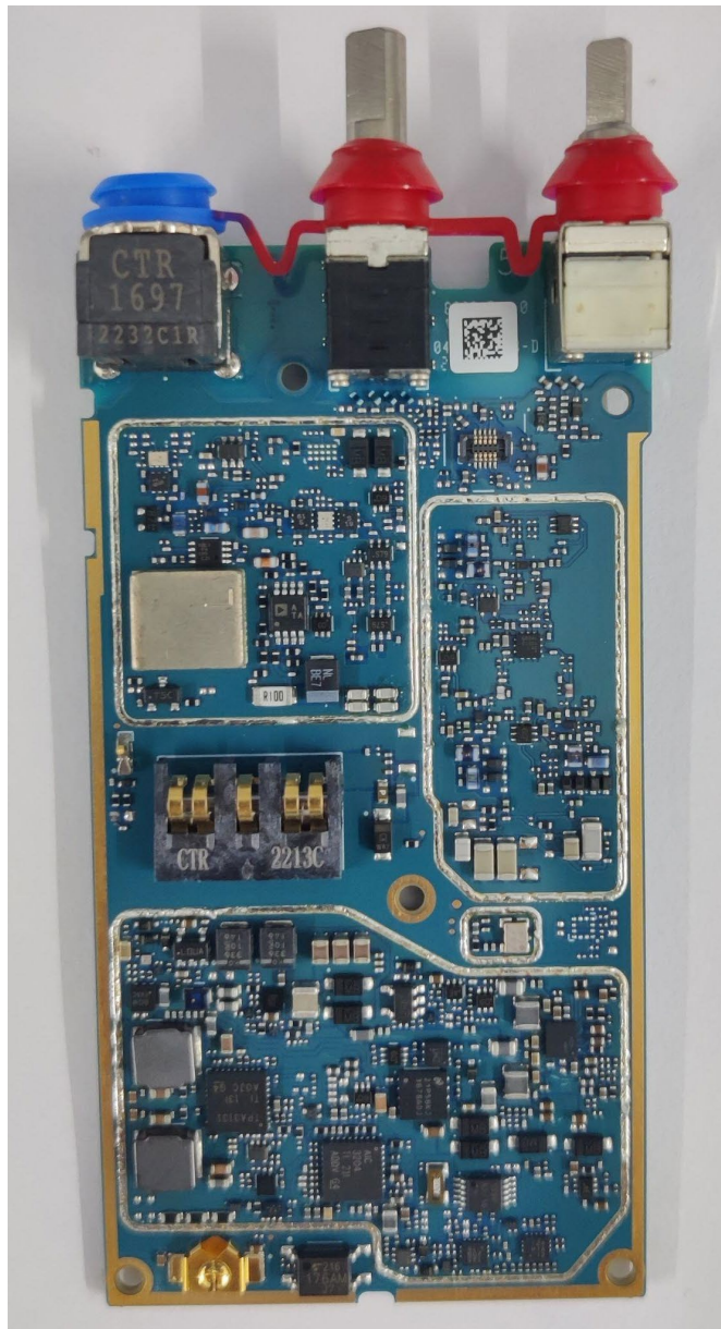
RF board without Shields (Bottom) of TIA NKP Model
