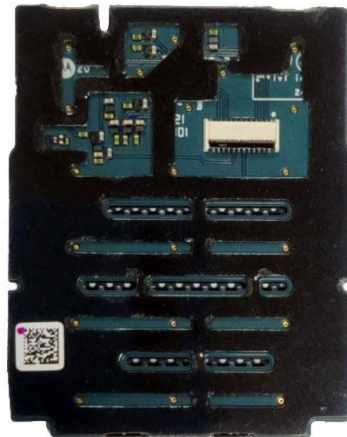
Keypad board (Bottom) of TIA FKP Model
