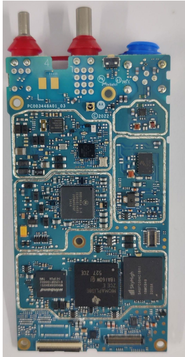
RF board without Shields (Top) of TIA NKP Model
