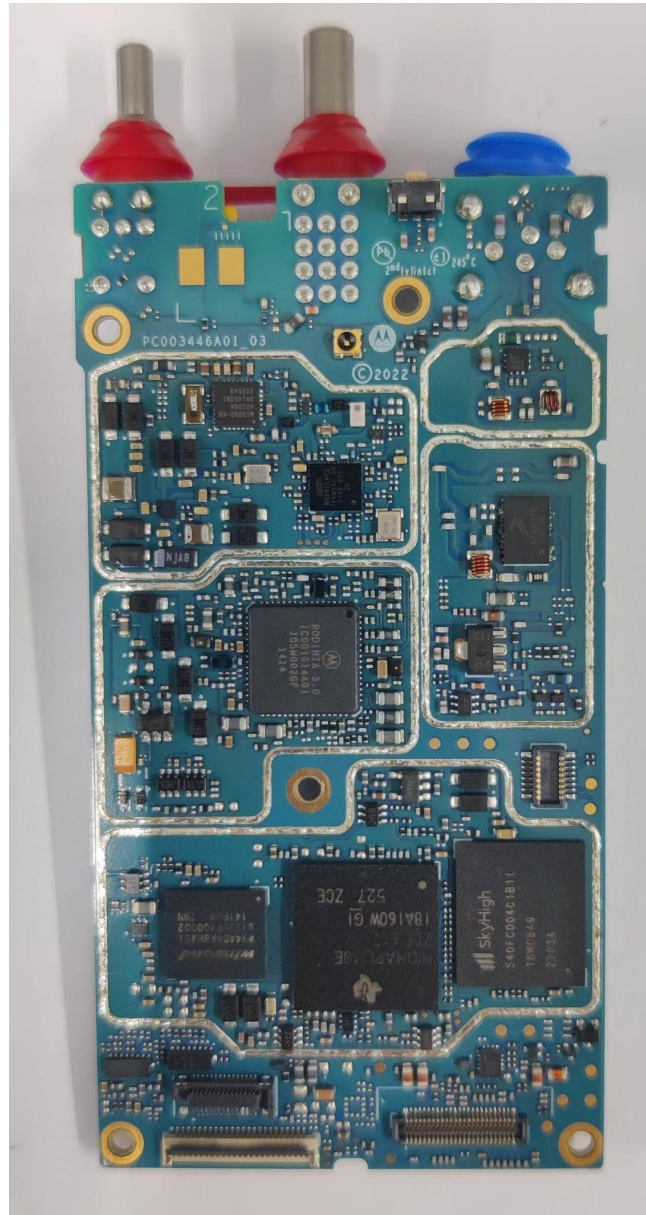
RF board without Shields (Top) of TIA FKP Model
