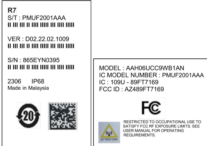
Figure 1G: AAH06UCC9WB1AN (IC Model: PMUF2001AAA)
