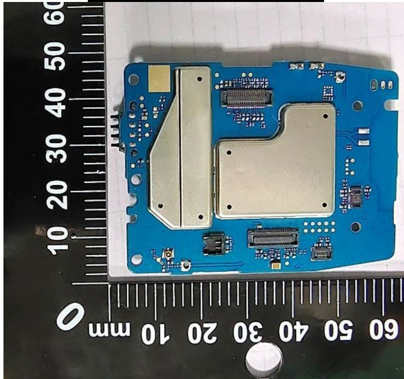
RF board with Shields (Bottom)
