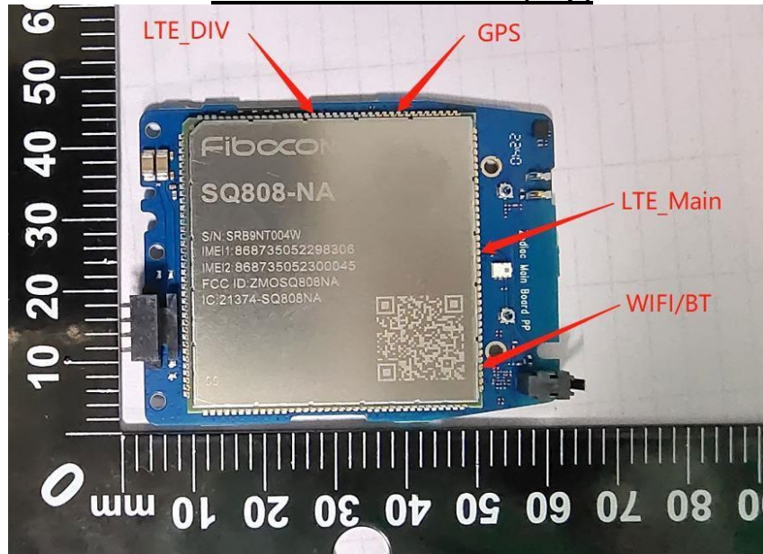
RF board with Shields (Top)
