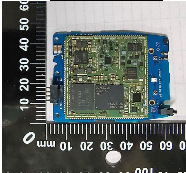
RF board without Shields (Top)
