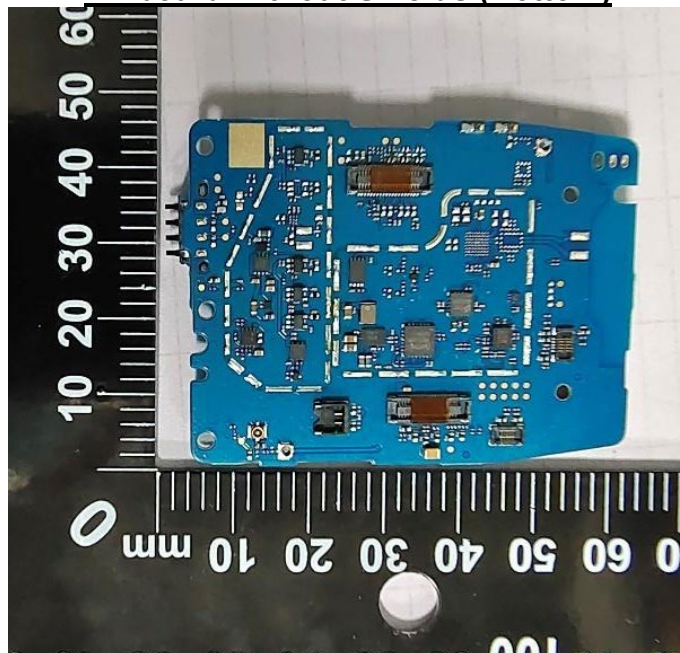
RF board without Shields (Bottom)
