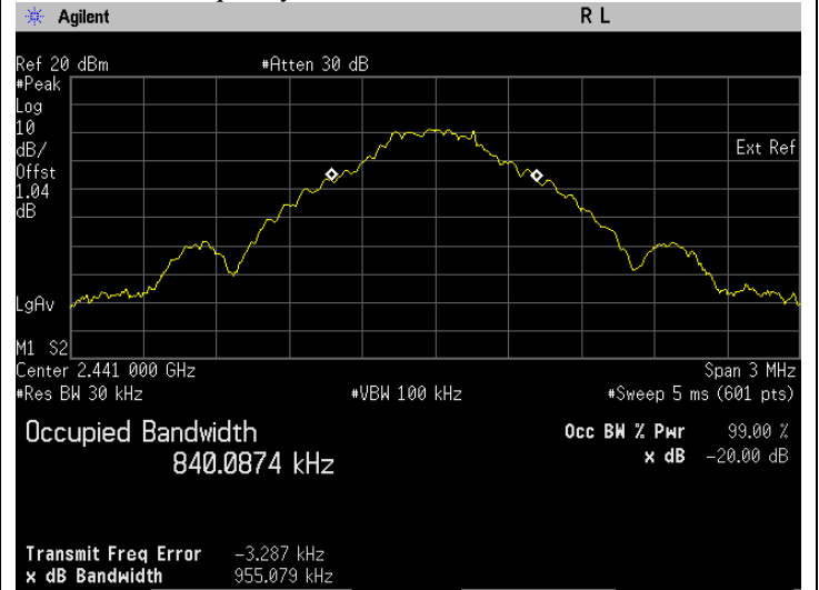
ii. The 20 dB BW & occupied bandwidth test with result at mid frequency, GFSK.
