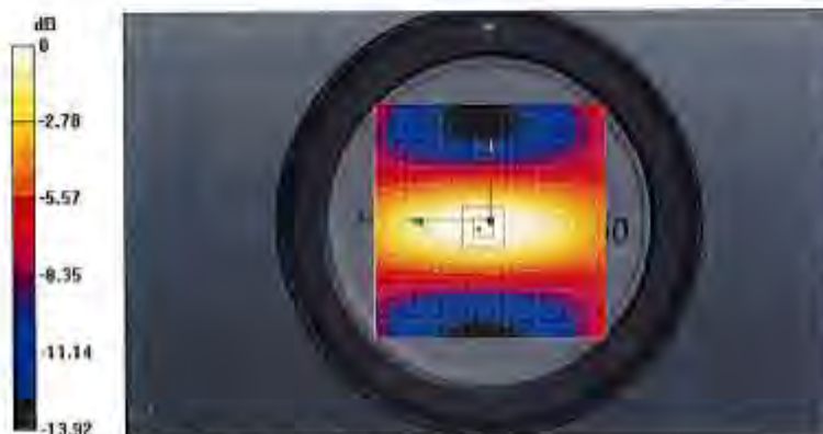
0 dB = 5.23 W/kg = 7.19 dBW/kg
