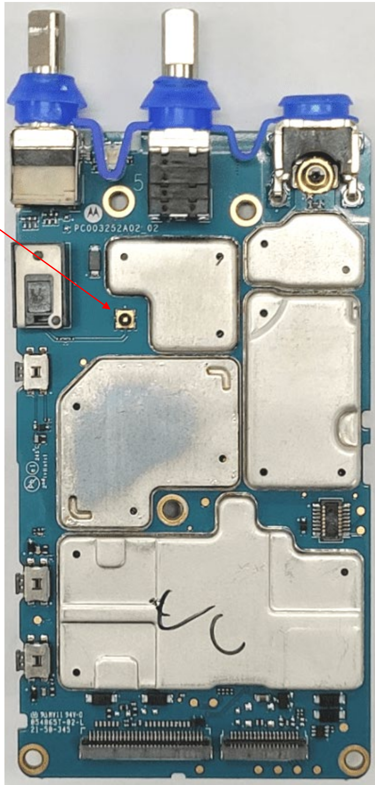
RF board with Shields (Top) TIA4950
