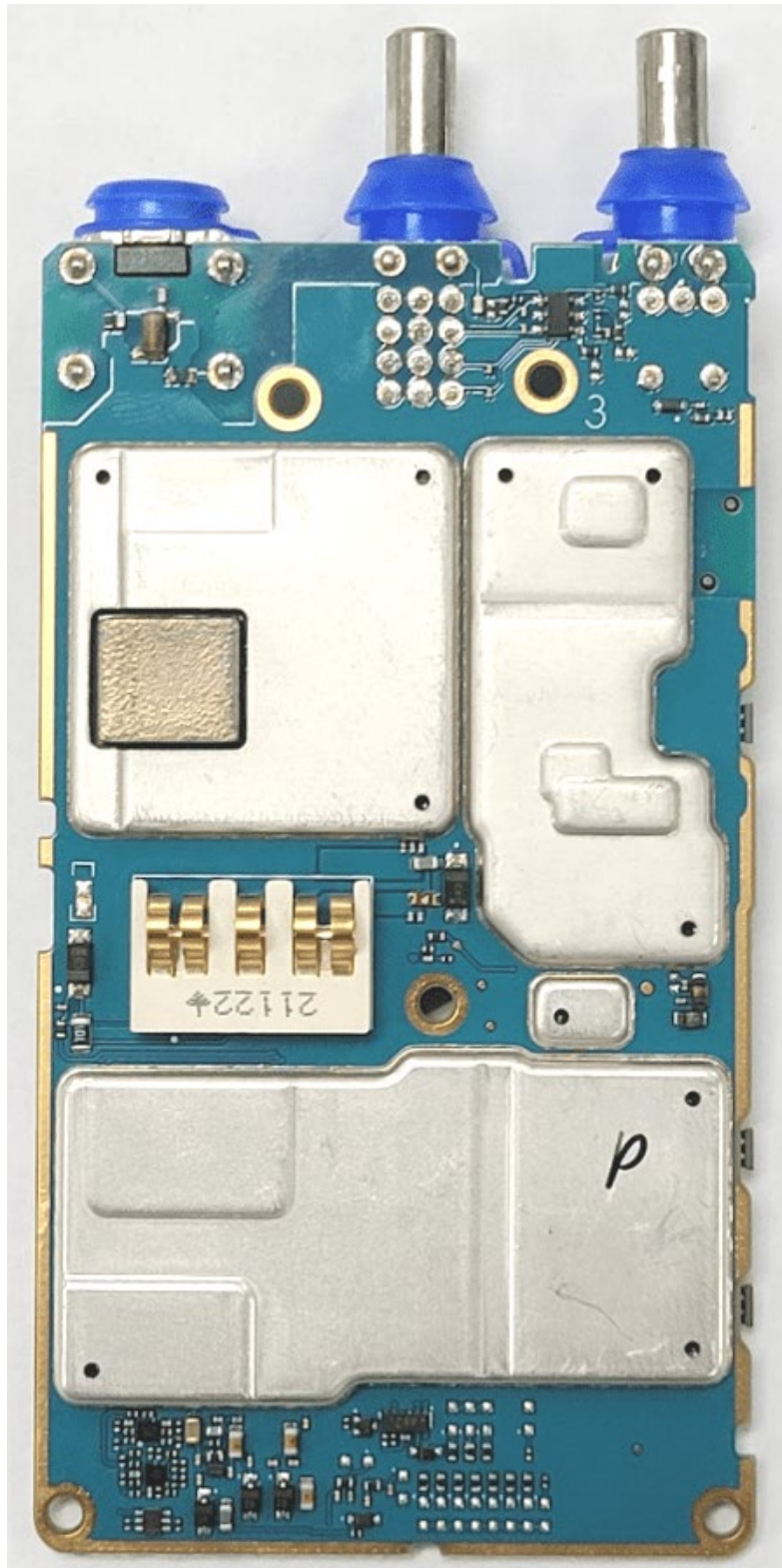
RF board with Shields (Bottom) Non-TIA4950
