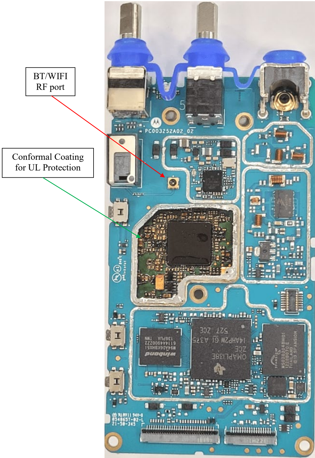
RF board without Shields (Top) TIA4950
