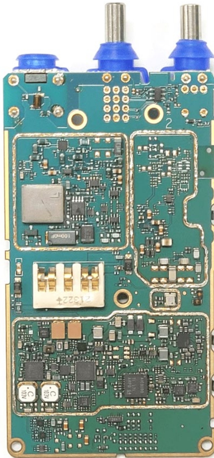
RF board without Shields (Bottom) Non-TIA4950
