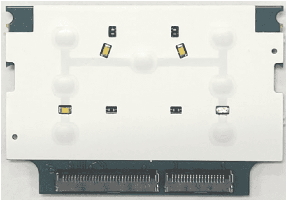
Limited Keypad Board (Top)
