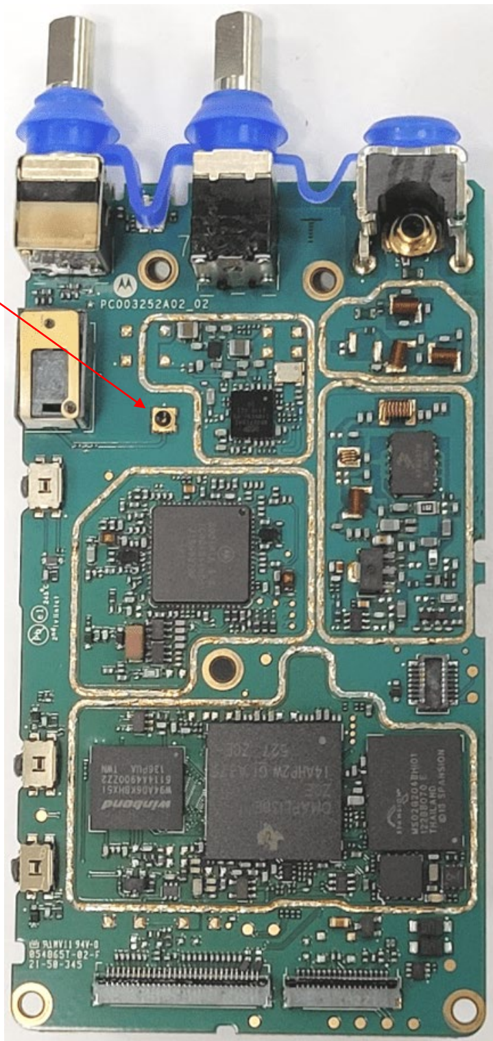
RF board without Shields (Top) Non-TIA4950
