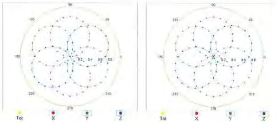
f=600 MHz,TEM
