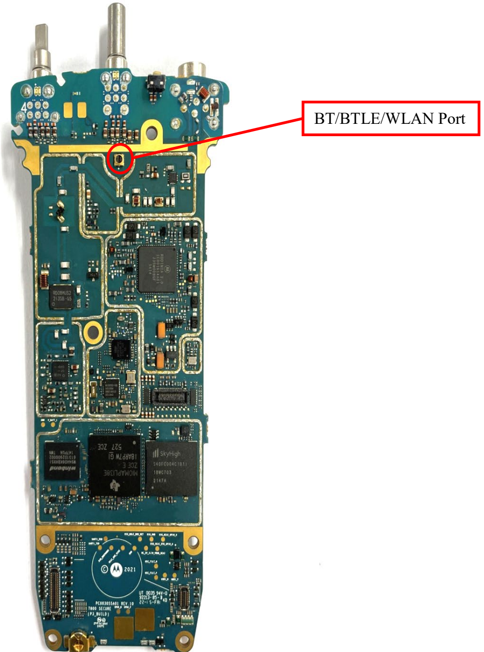
Main board without Shields (Top) (APX N50)
