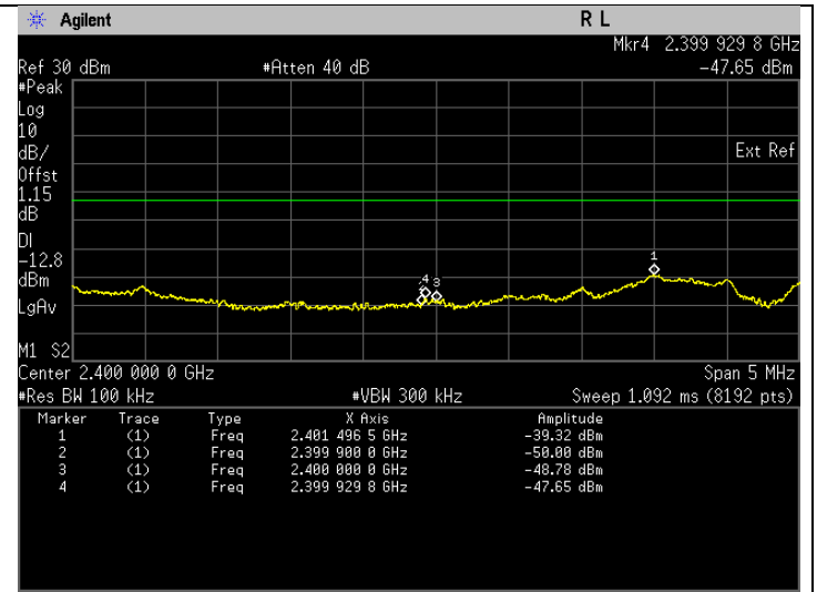
Band Edge(Peak). 802.11b Frequency 2412 MHz Band Edge
