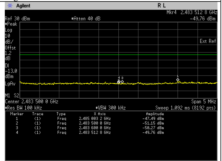
Band Edge(Peak). 802.11b Frequency 2462 MHz Band Edge
