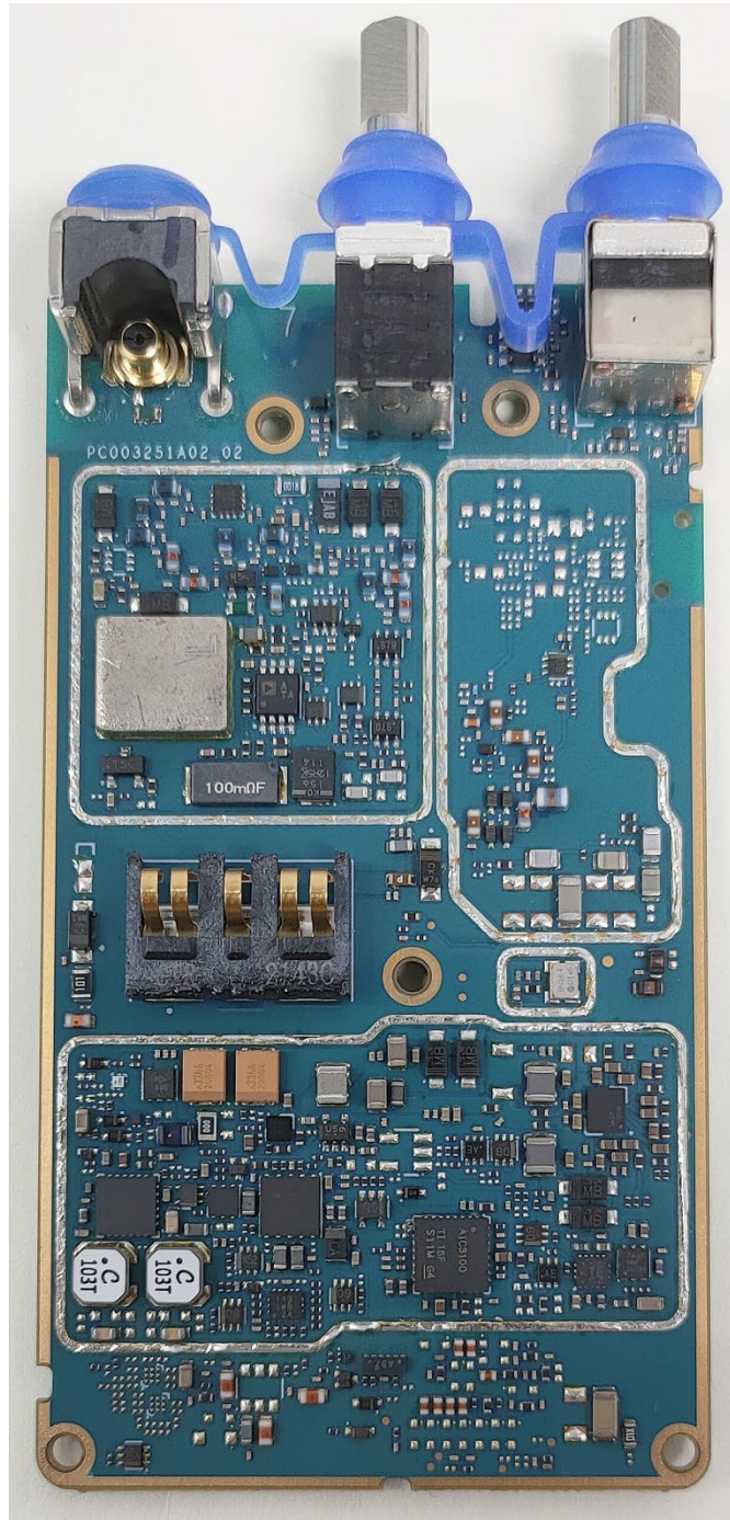
RF Board Without Shields (Bottom) TIA4950
