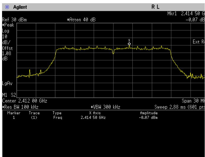
Conducted Emissions(Average). 802.11n, Frequency 2412 MHz Reference Level
