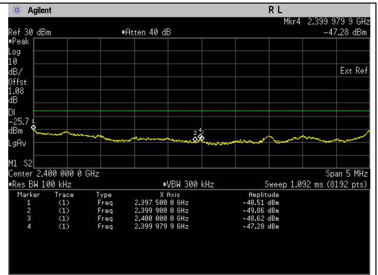
Band Edge(Average). 802.11b Frequency 2412 MHz Band Edge
