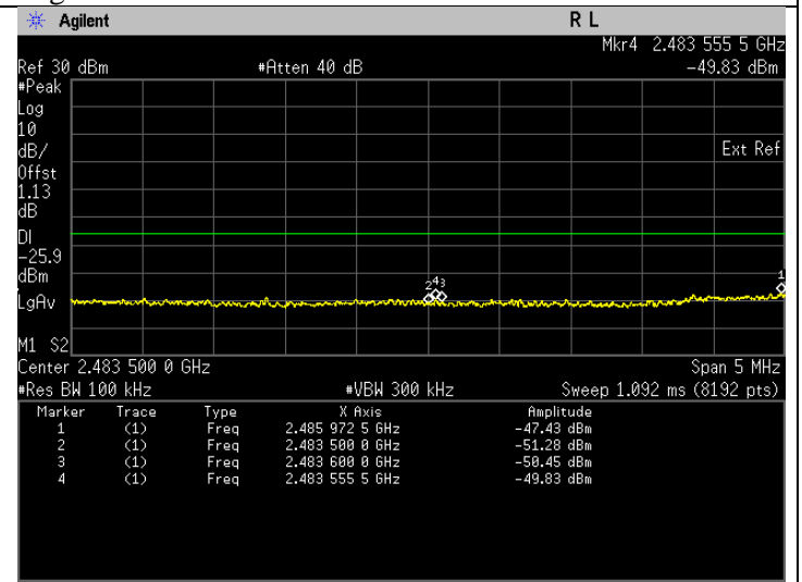
Band Edge(Average). 802.11b Frequency 2462 MHz Band Edge
