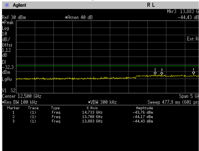
Conducted Emissions(Average). 802.11g, Frequency 2437 MHz Emission Level, 10 GHz -> 15 GHz
