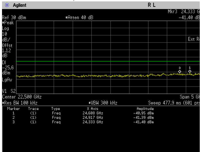
Conducted Emissions(Average). 802.11b, Frequency 2437 MHz Emission Level, 20 GHz -> 25 GHz
