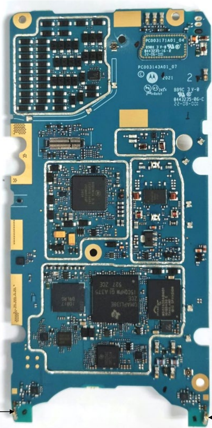
Exhibit 9D: LMR RF board without Shields (Top)
