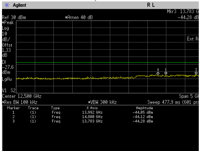
Conducted Emissions(Average). 802.11b, Frequency 2462 MHz Emission Level, 10 GHz -> 15 GHz
