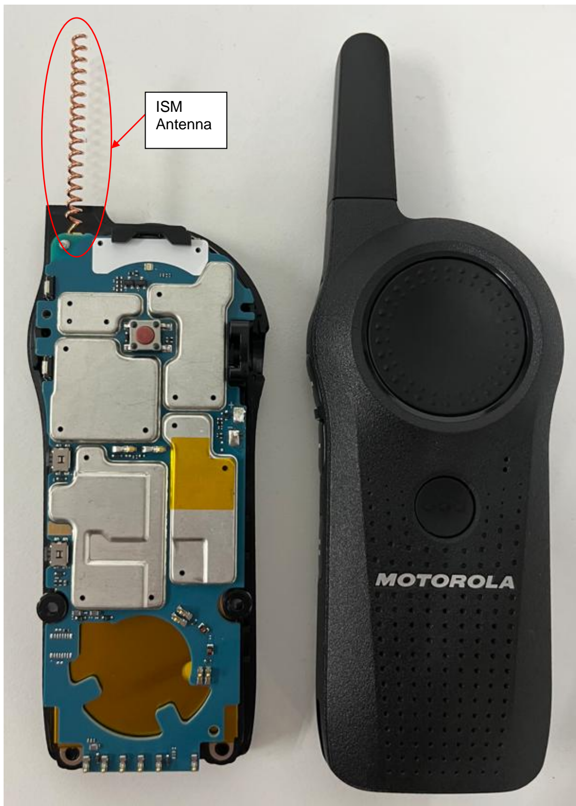
EXHIBIT 9E - RF board with chassis and housing (front side)
