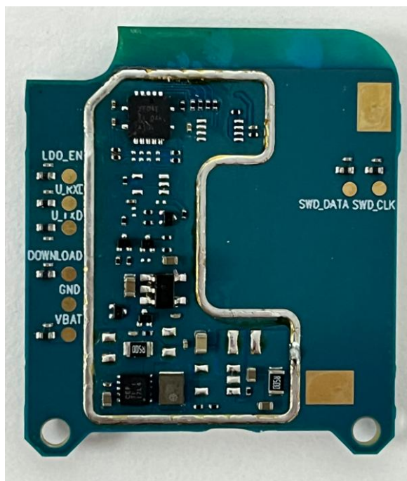
EXHIBIT 9H - WIFI board without Shields (Top)
