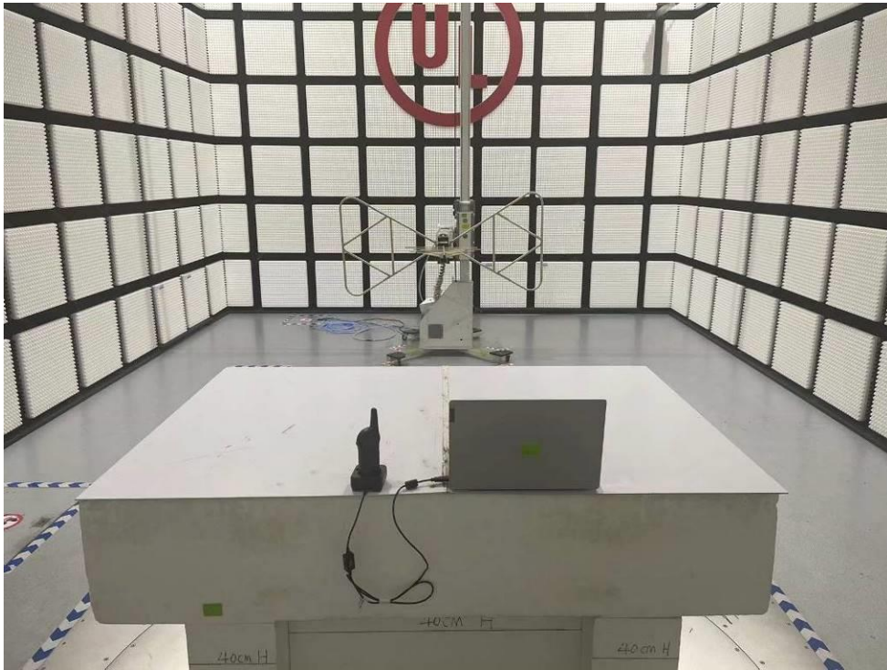
RADIATED SPURIOUS EMISSION SETUP ABOVE 1 GHz
