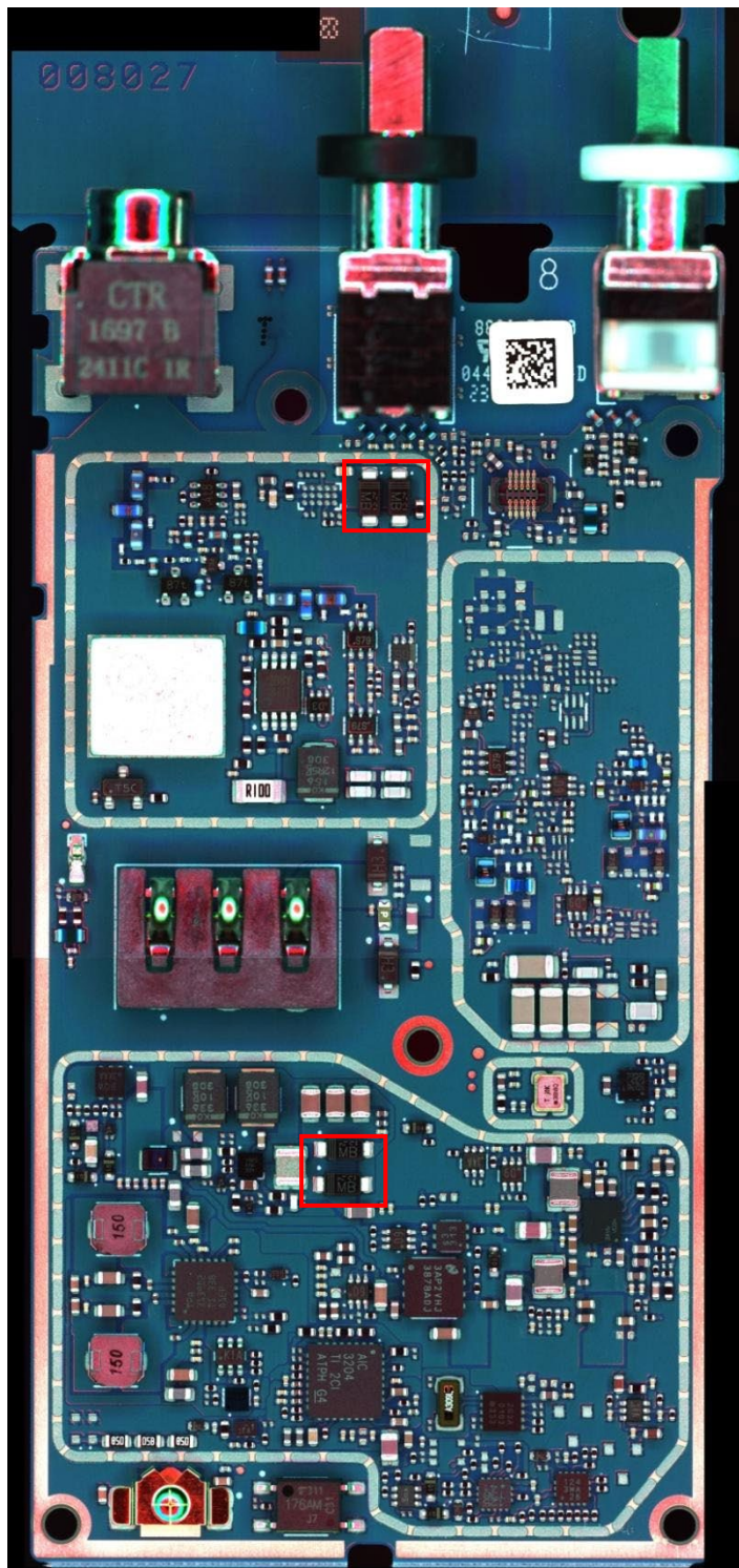
RF board without Shields (Bottom) of FKP TIA Model
