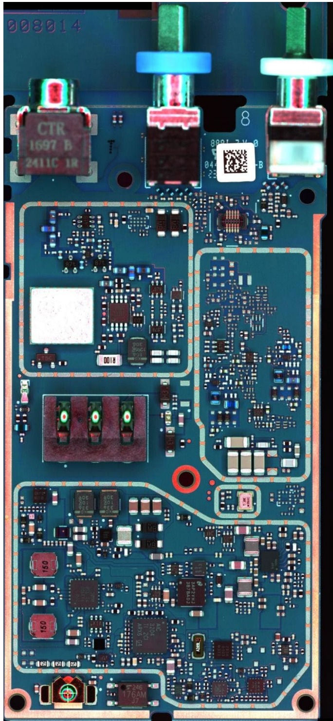
RF board without Shields (Bottom) of NKP TIA Model
