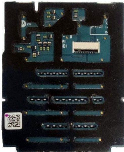
Keypad board (Bottom) of FKP TIA/non-TIA Model
