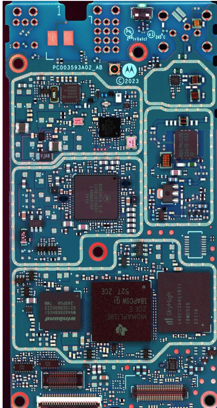
RF board without Shields (Top) of FKP non-TIA Model
