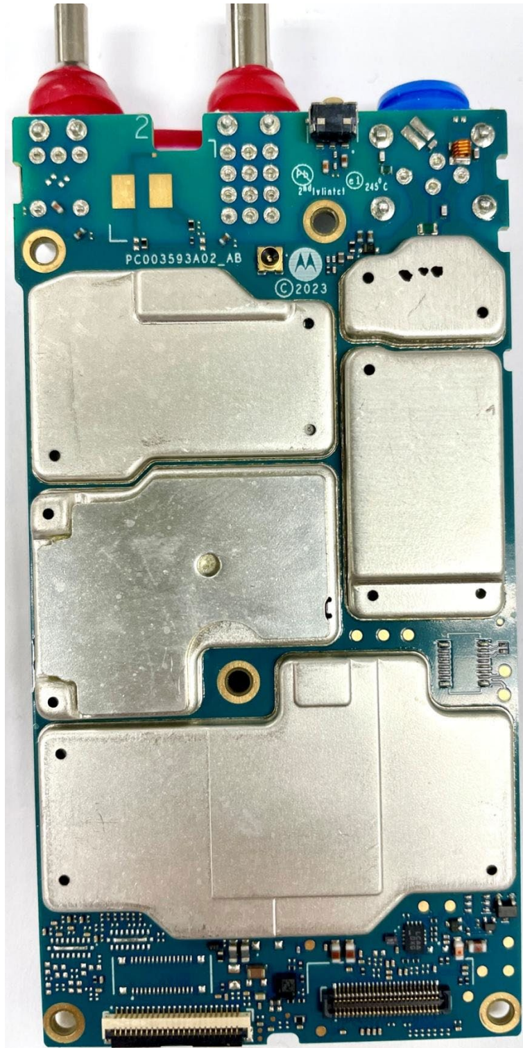
RF board with Shields (Top) of NKP TIA Model
