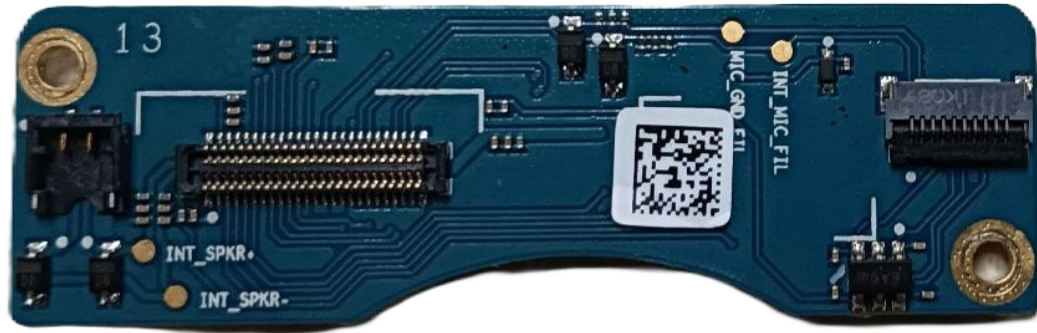
Interface board (Top)
