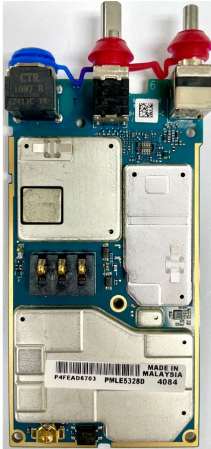
RF board with Shields (Bottom) of FKP TIA/non-TIA Model
