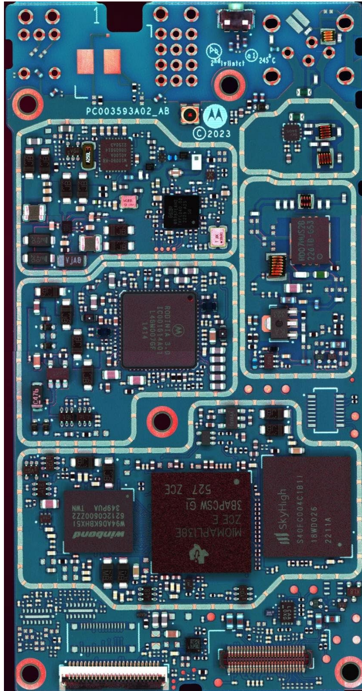
RF board without Shields (Top) of NKP TIA Model
