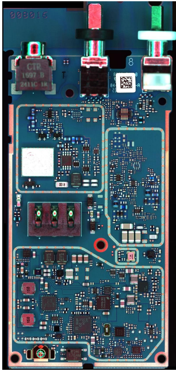
RF board without Shields (Bottom) of FKP non-TIA Model
