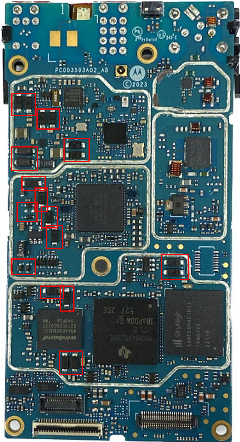
RF board without Shields (Top) of FKP TIA Model
