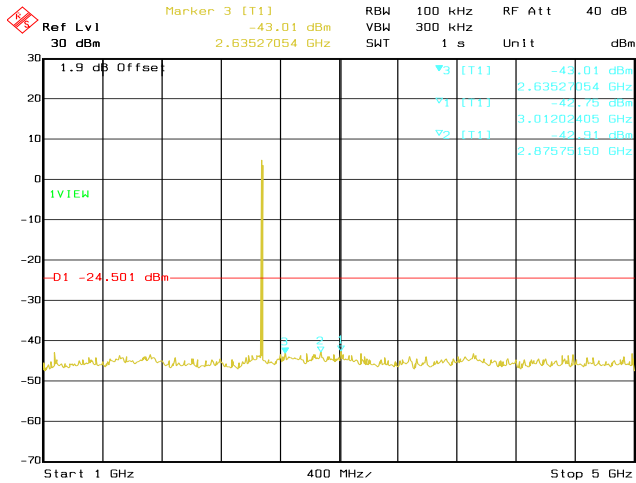
Date: 14.AUG.2020 03:18:32 Conducted Emissions. Bluetooth LE, Frequency 2480 MHz Emission Level, 1 GHz -> 5 GHz
