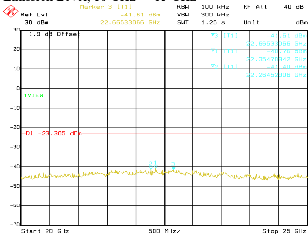
Conducted Emissions. Bluetooth LE, Frequency 2440 MHz Emission Level, 20 GHz -> 25 GHz
