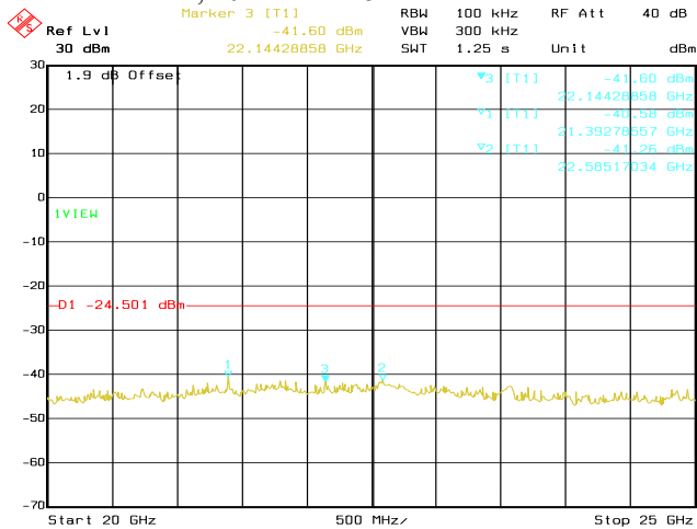
Date: 14.AUG.2020 03:22:04 Conducted Emissions. Bluetooth LE, Frequency 2480 MHz Emission Level, 20 GHz -> 25 GHz
