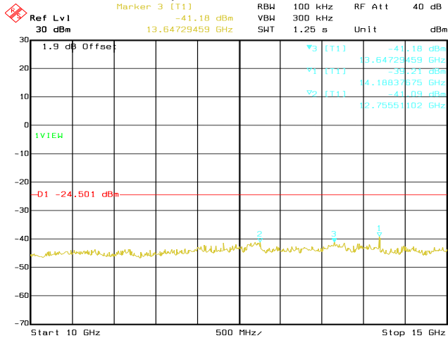
Date: 14.AUG.2020 03:20:18 Conducted Emissions. Bluetooth LE, Frequency 2480 MHz Emission Level, 10 GHz -> 15 GHz
