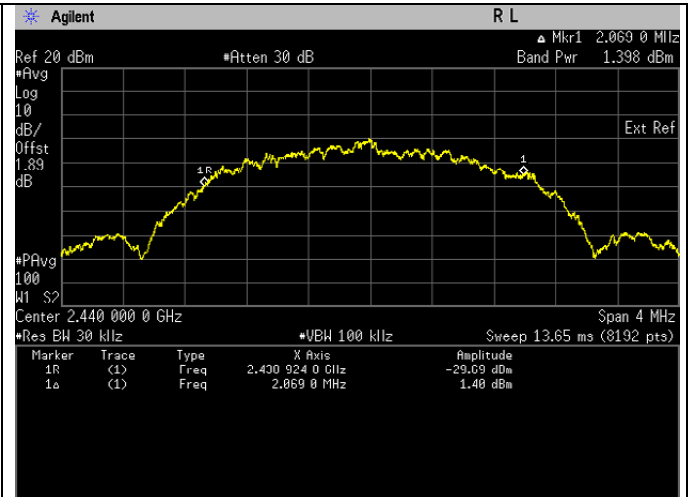
Frequency 2440 MHz
