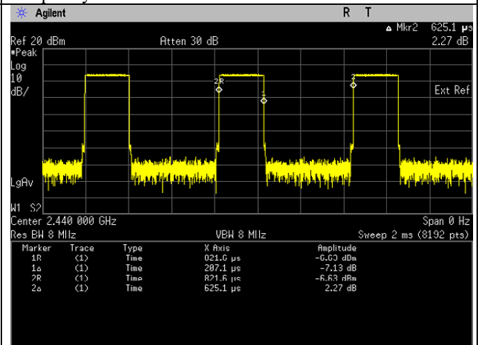
Duty Cycle
