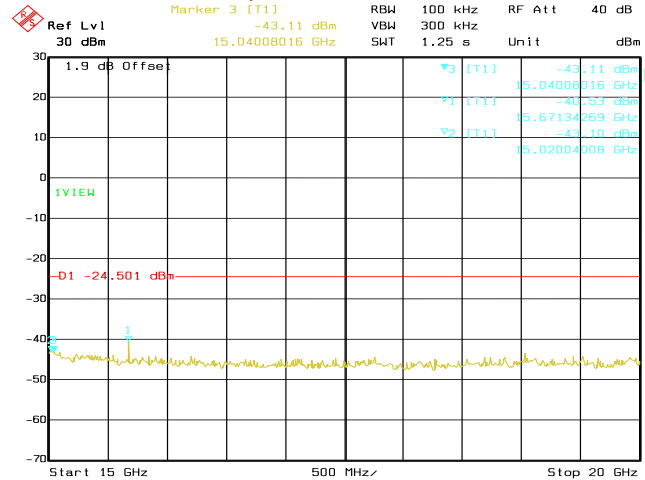
Date: 14.AUG.2020 03:21:11 Conducted Emissions. Bluetooth LE, Frequency 2480 MHz Emission Level, 15 GHz -> 20 GHz
