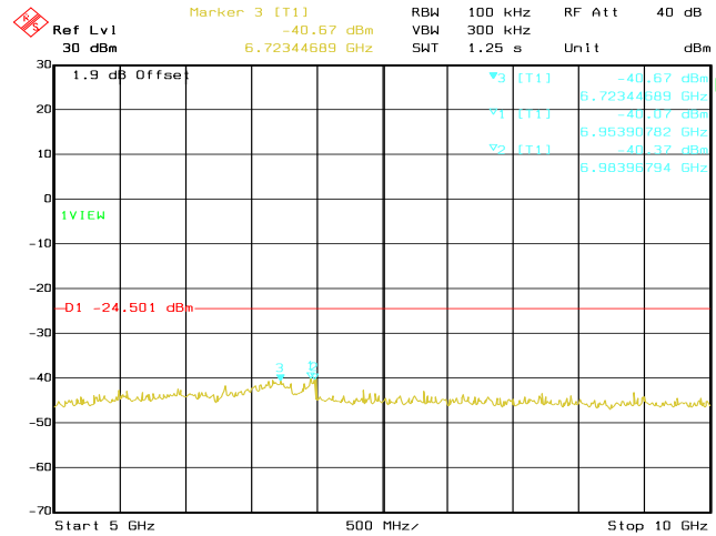
Date: 14.AUG.2020 03:19:25 Conducted Emissions. Bluetooth LE, Frequency 2480 MHz Emission Level, 5 GHz -> 10 GHz
