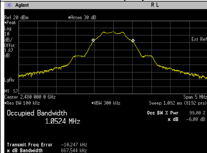
6dB Bandwidth. Bluetooth LE Frequency 2480 MHz
