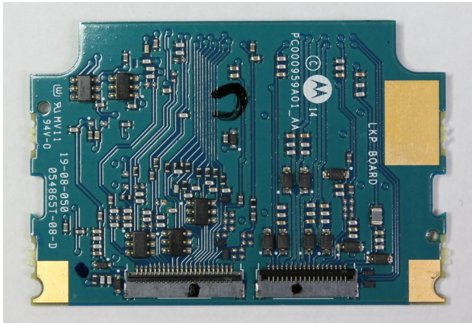
Limited Keypad board (Bottom)
