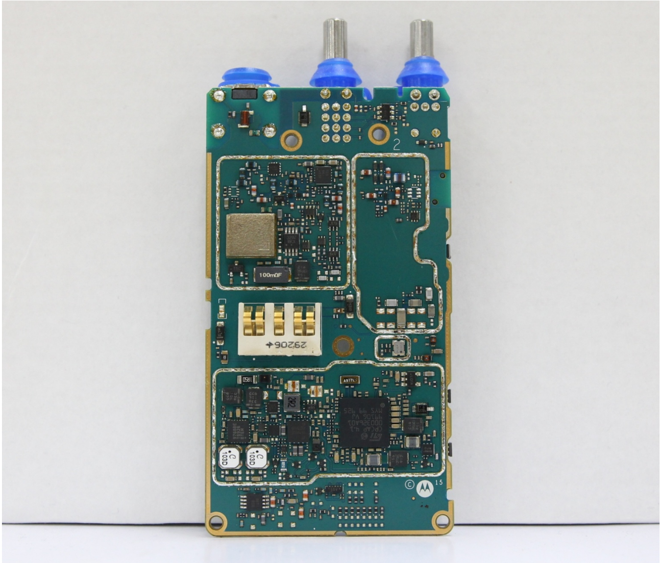
RF board without Shields (Bottom)
