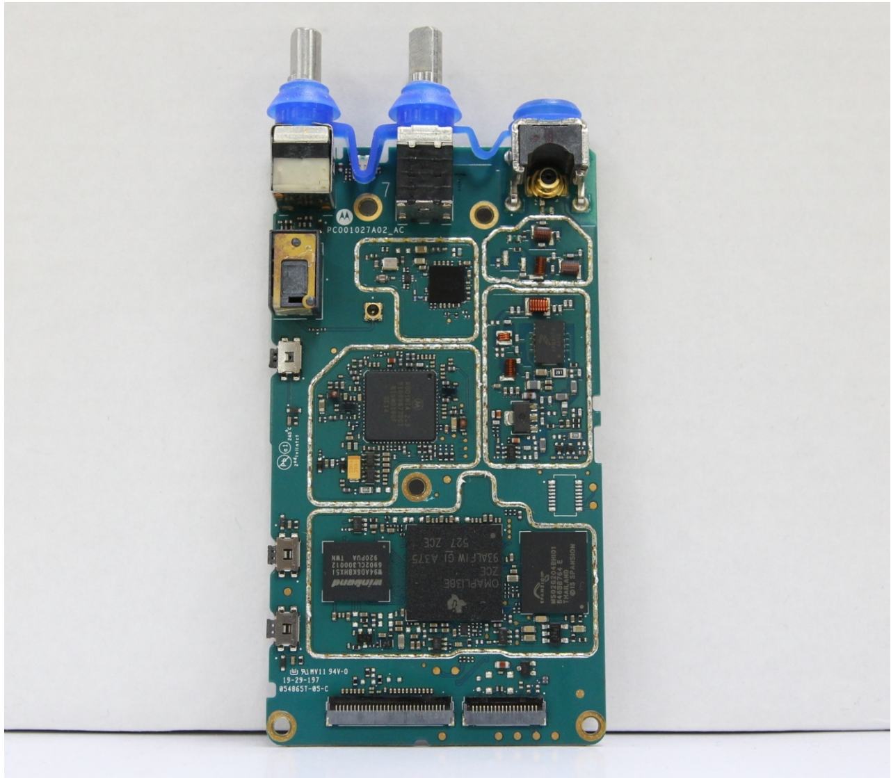
RF board without Shields (Top)
