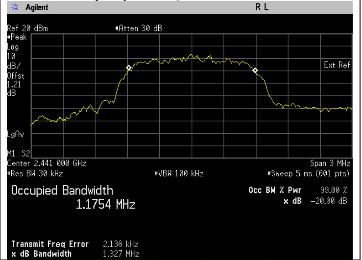
ii. The 20 dB BW & occupied bandwidth test with result at mid frequency, Pi/4 DQPSK.
