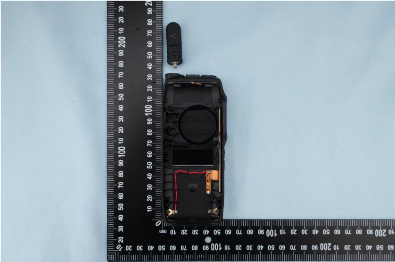
<Device disassembled LTE main antenna>
