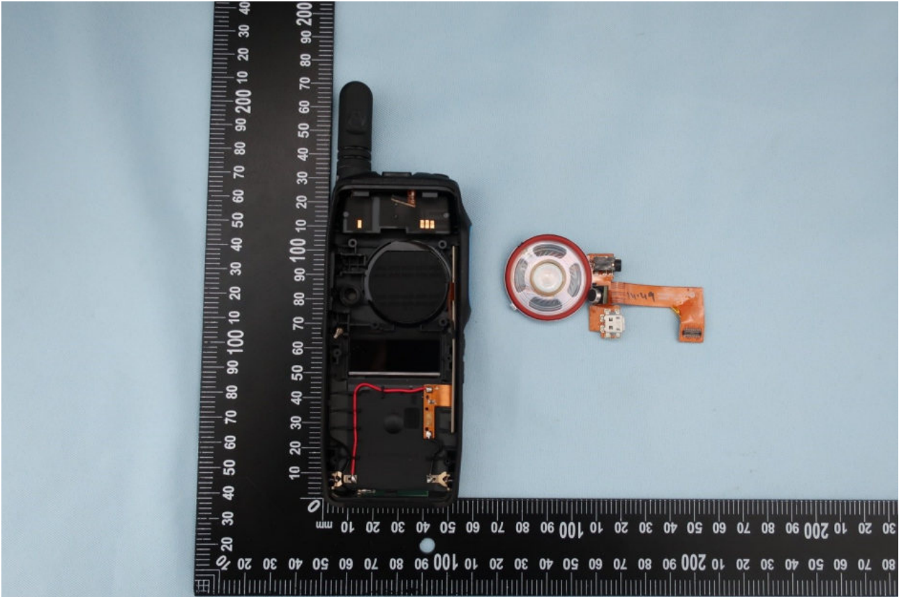
<Device disassembled speaker_mic_USB_audiojack FPCA>
