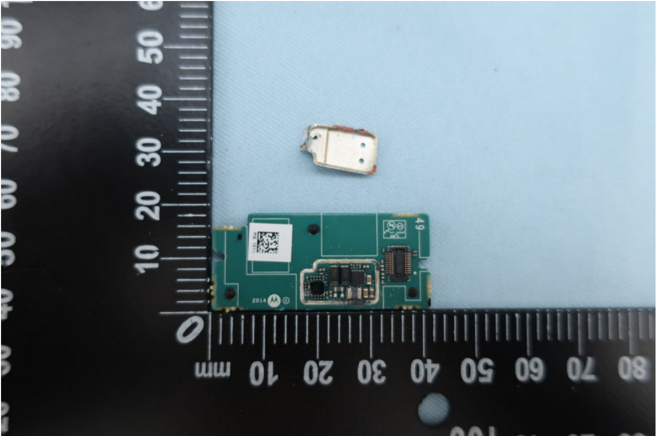
<Display PCBA bottom side remove shielding can>
