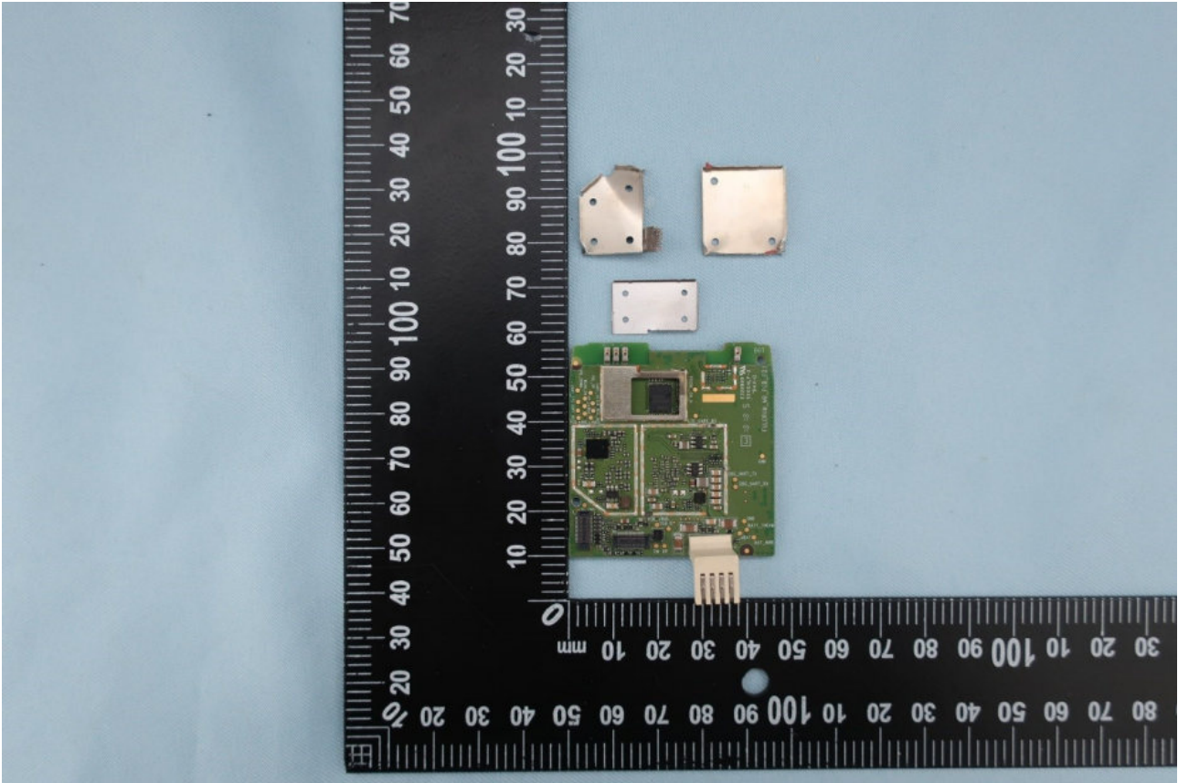
<Main PCBA top side remove shielding can>
