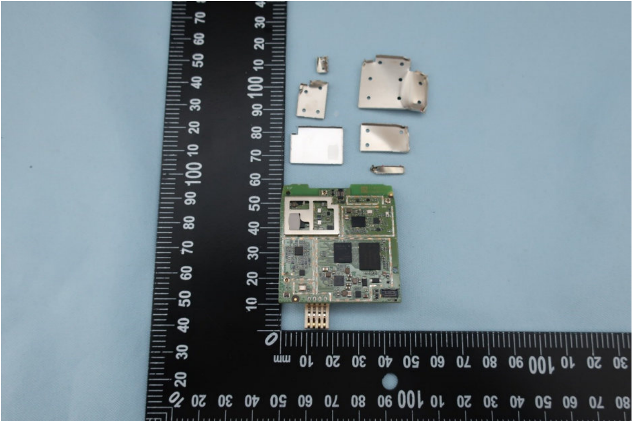
<Main PCBA bottom side remove shielding can>
