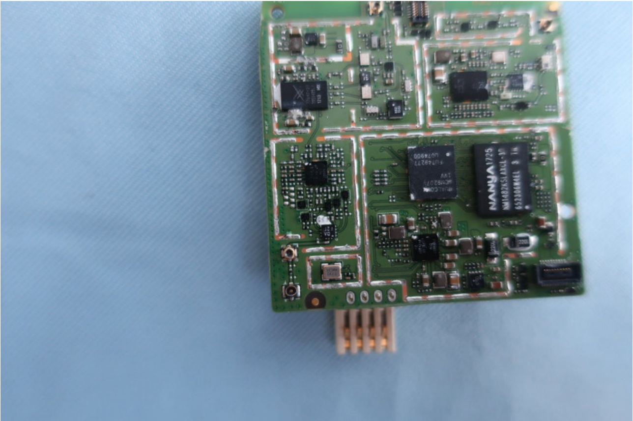
<Main PCBA top side without shielding can>
