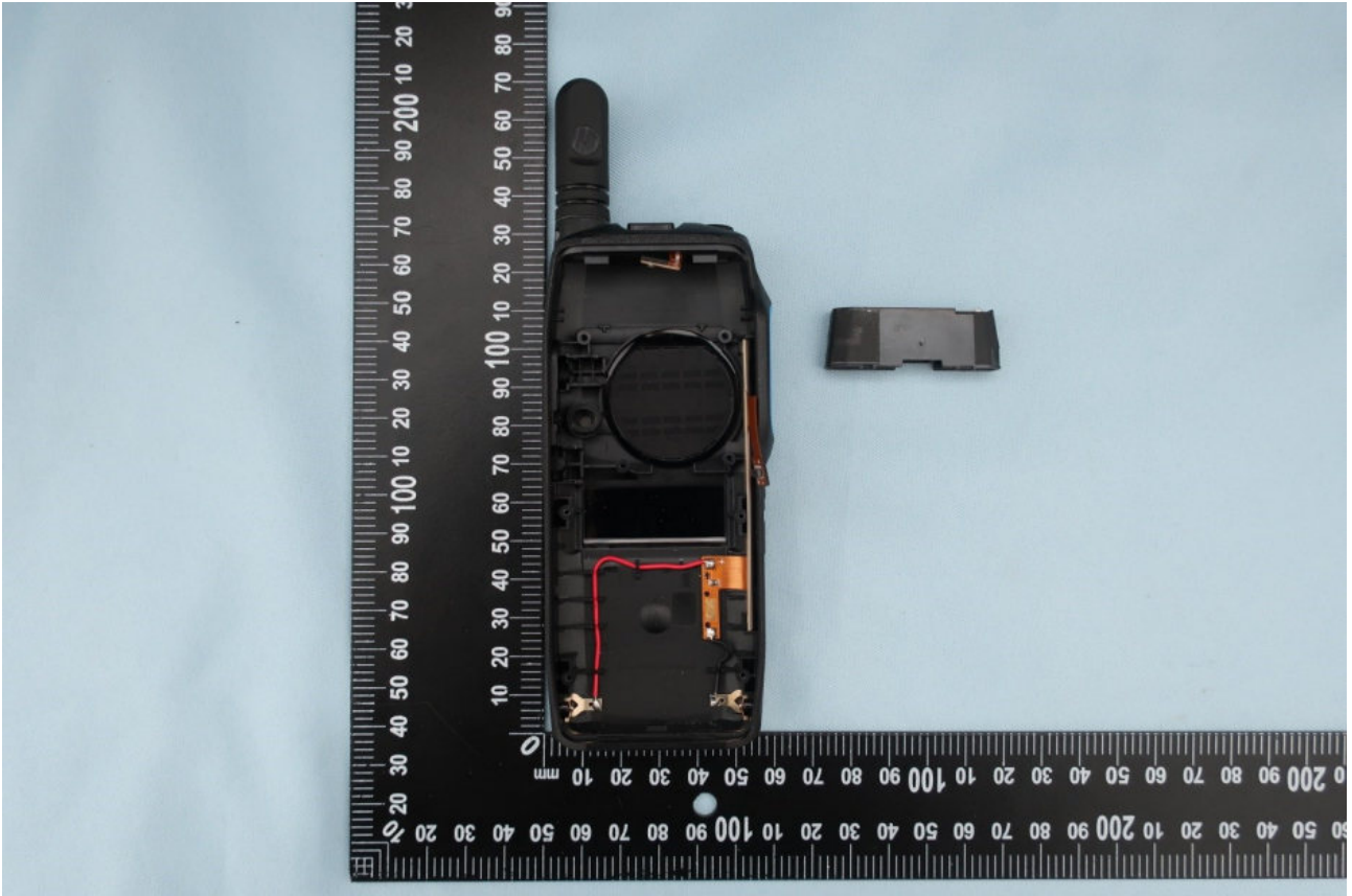
<Device disassembled GPS/WIFI/BT antenna frame>
