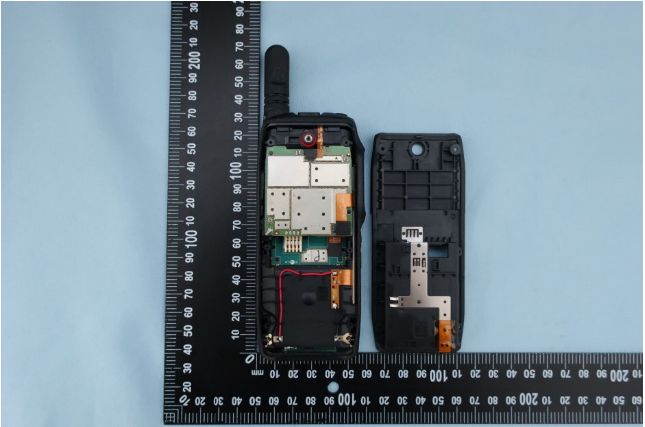
<Device disassembled rear housing>
