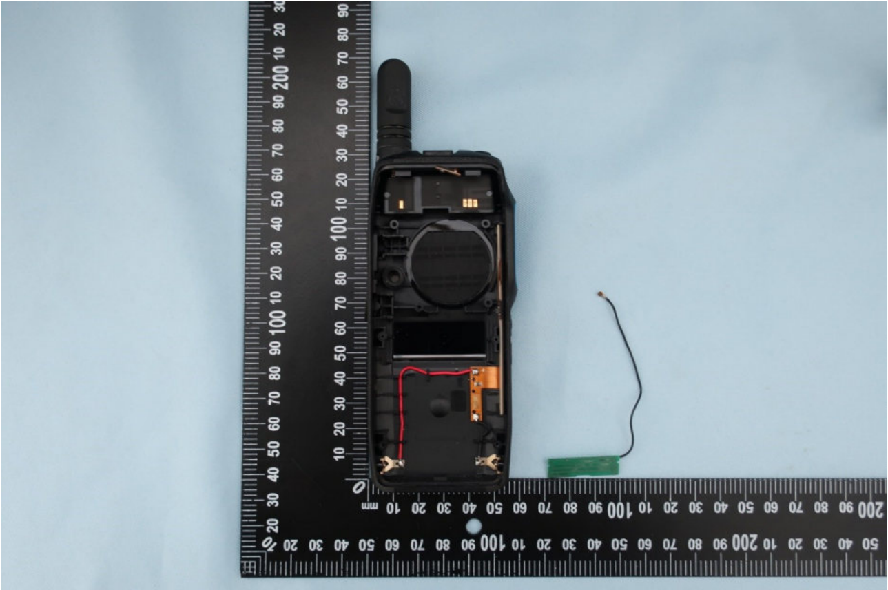
<Device disassembled LTE diversity antenna>
