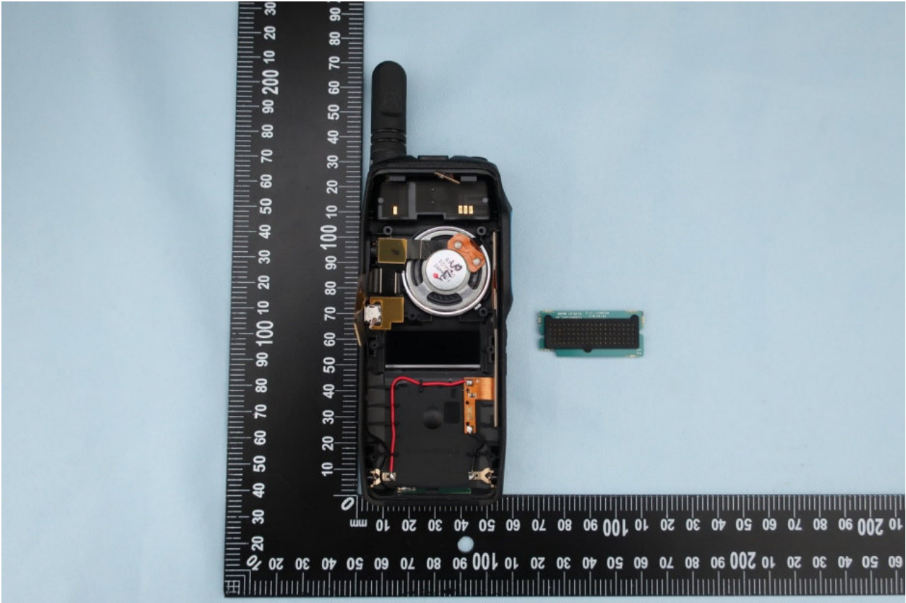
<Device disassembled display PCBA>
