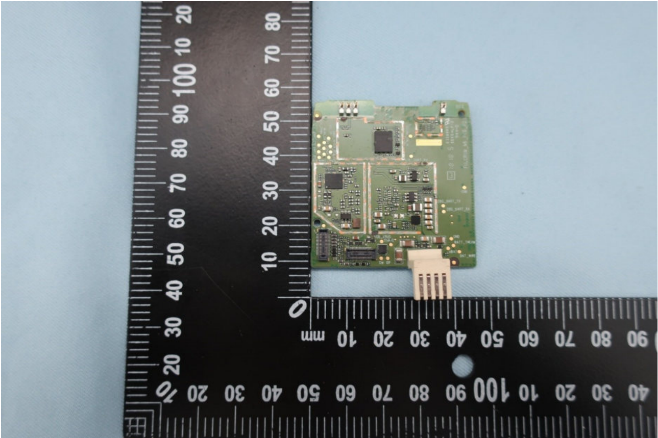
<Main PCBA top side remove shielding frame>
