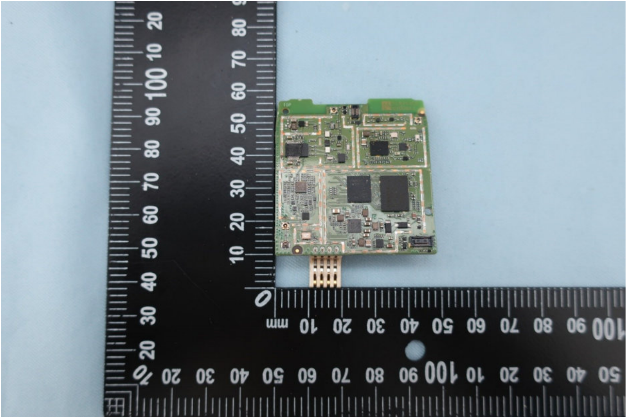
<Main PCBA bottom side remove shielding frame>
