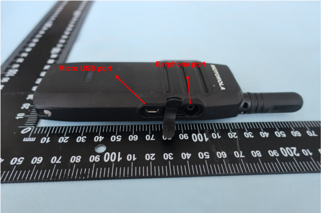
<External port>
