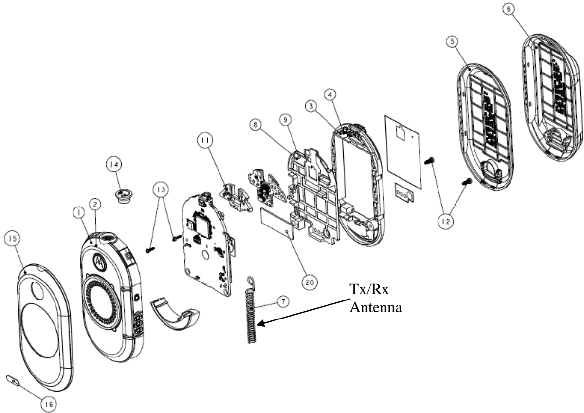
Exploded View of Radio
