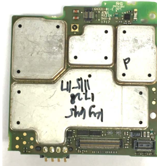
RF board with Shields (Bottom)
