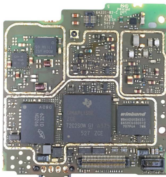
RF board without Shields (Bottom)
