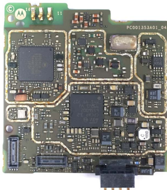
RF board without Shields (Top)
