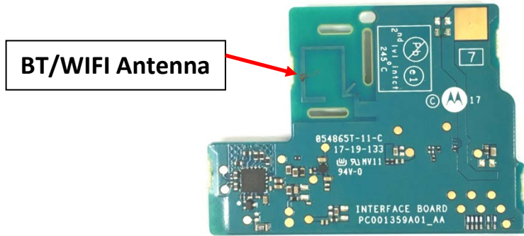
WIFI Board (Top)
