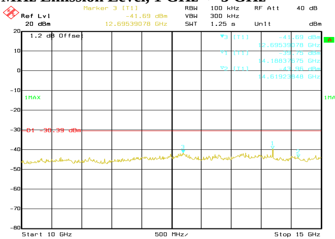
Conducted Emissions. 802.11n, Frequency 2462 MHz Emission Level, 10 GHz -> 15 GHz
