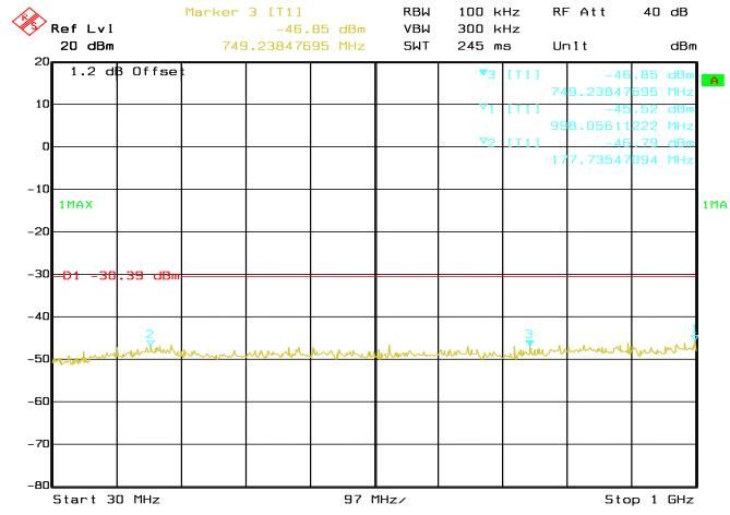
Conducted Emissions. 802.11n, Frequency 2462 MHz Emission Level, 30 MHz -> 1 GHz
