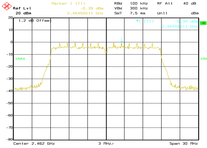
Conducted Emissions. 802.11n, Frequency 2462 MHz Reference Level
