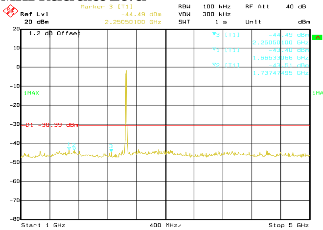
Conducted Emissions. 802.11n, Frequency 2462 MHz Emission Level, 1 GHz -> 5 GHz
