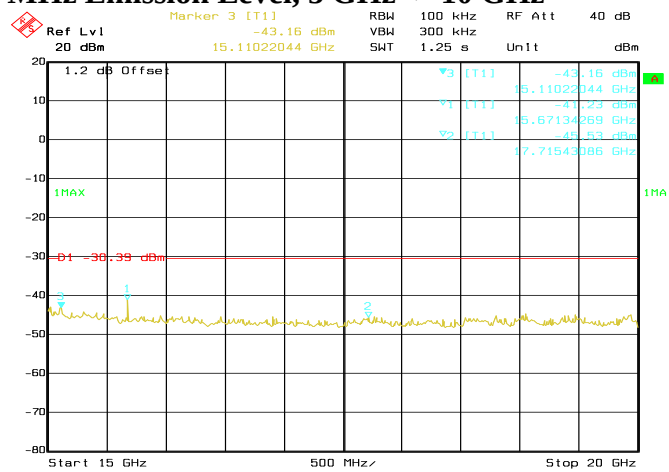
Conducted Emissions. 802.11n, Frequency 2462 MHz Emission Level, 15 GHz -> 20 GHz
