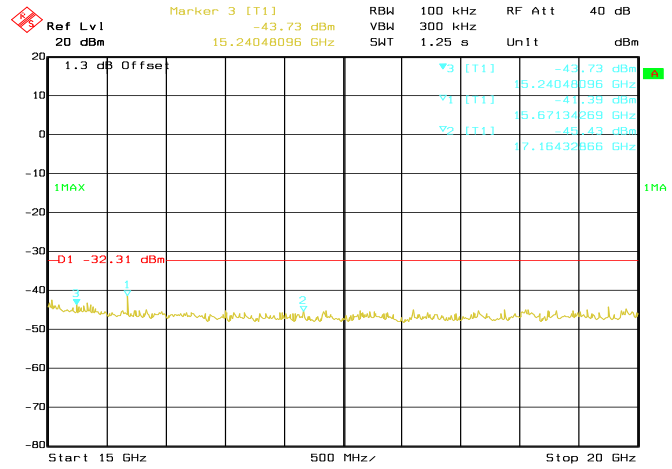
Conducted Emissions. 802.11g, Frequency 2412 MHz Emission Level, 15 GHz -> 20 GHz
