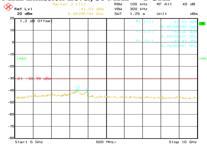
Conducted Emissions. 802.11n, Frequency 2462 MHz Emission Level, 5 GHz -> 10 GHz
