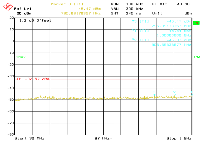
Conducted Emissions. 802.11g, Frequency 2437 MHz Emission Level, 30 MHz -> 1 GHz
