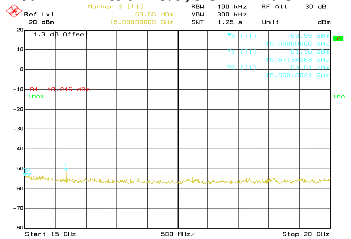
Conducted Emissions. Bluetooth LE, Frequency 2480 MHz Emission Level, 15 GHz -> 20 GHz
