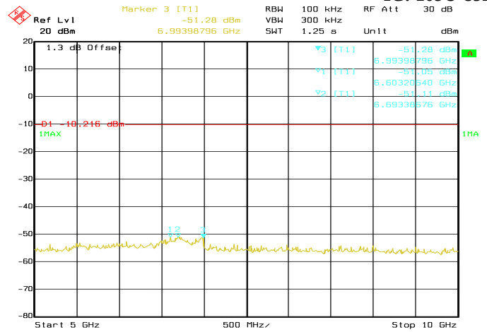
Date: 07.JUN.2017 19:28:57 Conducted Emissions. Bluetooth LE, Frequency 2480 MHz Emission Level, 5 GHz -> 10 GHz
