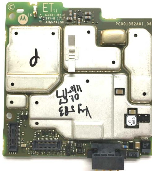
RF board with Shields (Top)
