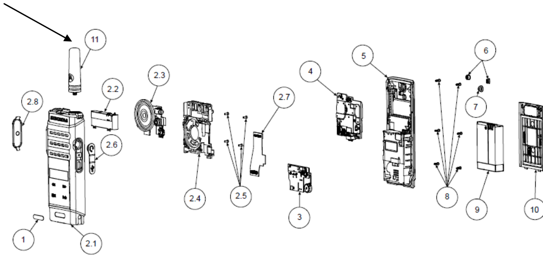
Exploded View of Radio
