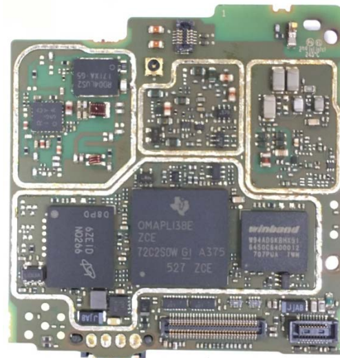
RF board without Shields (Bottom)
