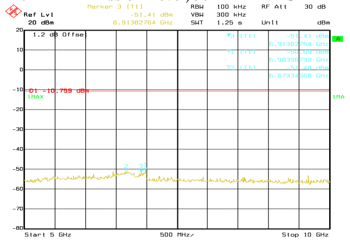
Date: 04.JUN.2017 11:10:17 Conducted Emissions. Bluetooth LE, Frequency 2402 MHz Emission Level, 5 GHz -> 10 GHz
