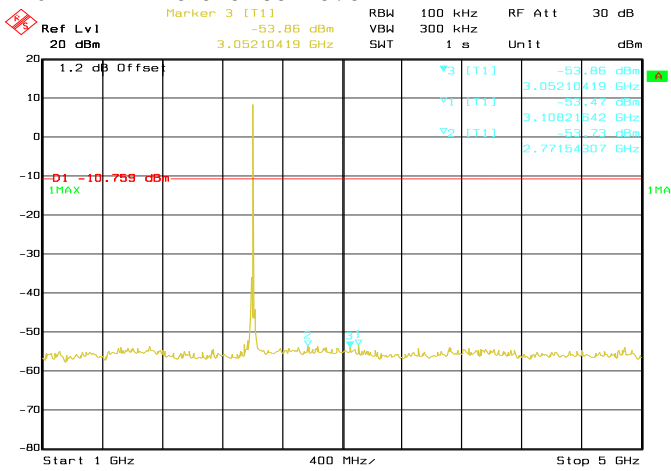
Date: 04.JUN.2017 11:09:44 Conducted Emissions. Bluetooth LE, Frequency 2402 MHz Emission Level, 1 GHz -> 5 GHz
