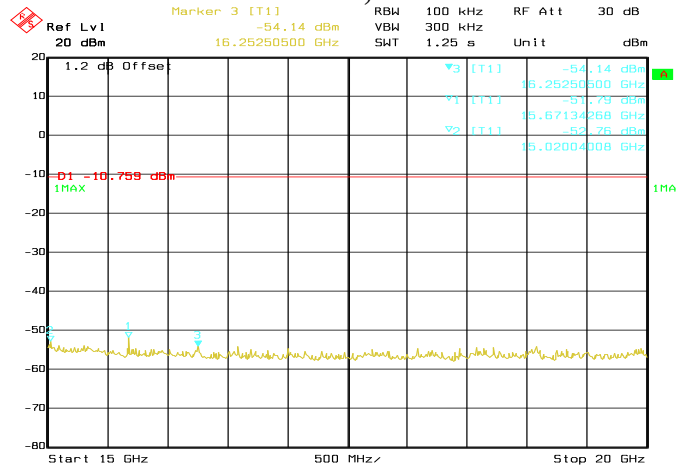
Date: 04.JUN.2017 11:11:23 Conducted Emissions. Bluetooth LE, Frequency 2402 MHz Emission Level, 15 GHz -> 20 GHz
