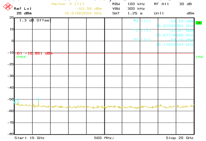
Date: 04 JUN 2017 11:20:28 Conducted Emissions. Bluetooth LE, Frequency 2480 MHz Emission Level, 15 GHz -> 20 GHz
