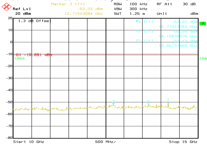
Date: 04 JUN 2017 11:19:55 Conducted Emissions. Bluetooth LE, Frequency 2480 MHz Emission Level, 10 GHz -> 15 GHz
