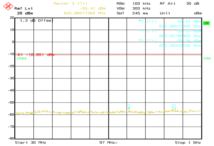
Conducted Emissions. Bluetooth LE, Frequency 2480 MHz Emission Level, 30 MHz -> 1 GHz
