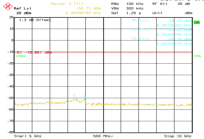
Date: 04 JUN 2017 11:19:22 Conducted Emissions. Bluetooth LE, Frequency 2480 MHz Emission Level, 5 GHz -> 10 GHz
