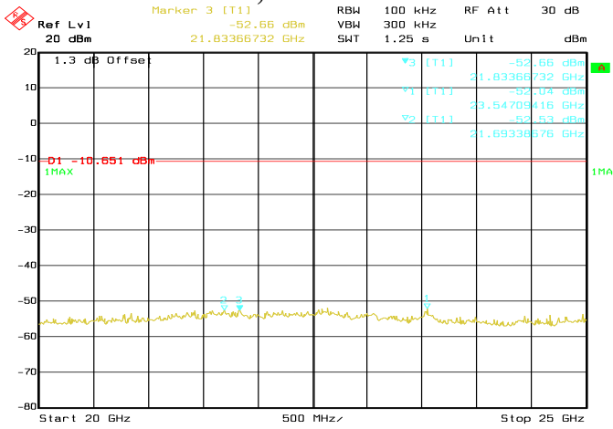
Date: 04 JUN 2017 11:21:00 Conducted Emissions. Bluetooth LE, Frequency 2480 MHz Emission Level, 20 GHz -> 25 GHz
