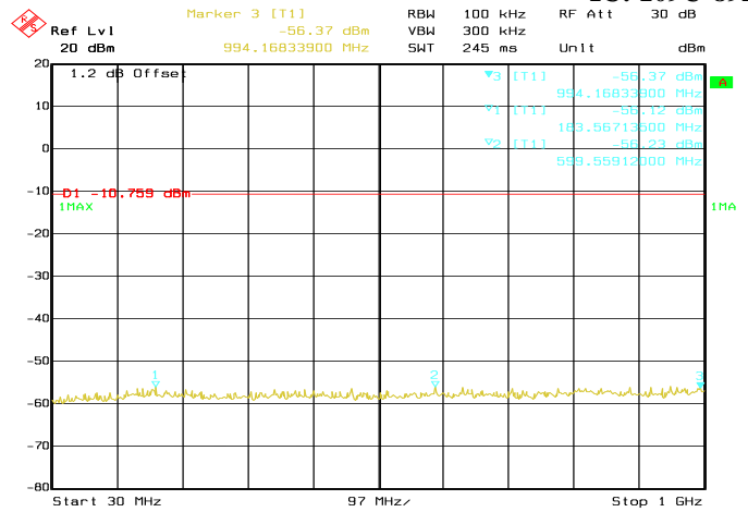
Date: 04.JUN.2017 11:09:12 Conducted Emissions. Bluetooth LE, Frequency 2402 MHz Emission Level, 30 MHz -> 1 GHz
