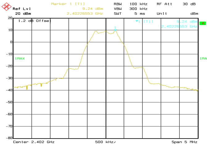
Date: 04.JUN.2017 11:08:39 Conducted Emissions. Bluetooth LE, Frequency 2402 MHz Reference Level
