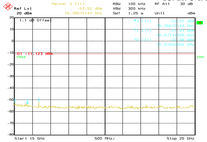
Conducted Emissions. Bluetooth LE, Frequency 2440 MHz Emission Level, 15 GHz -> 20 GHz
