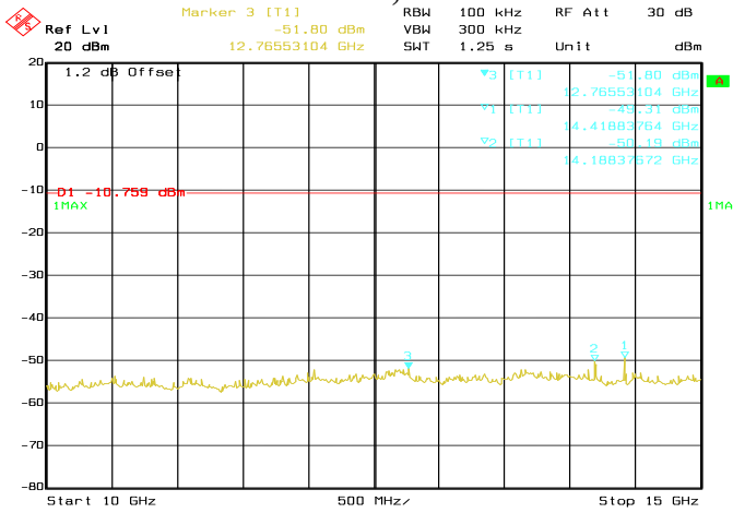
Date: 04.JUN.2017 11:10:50 Conducted Emissions. Bluetooth LE, Frequency 2402 MHz Emission Level, 10 GHz -> 15 GHz
