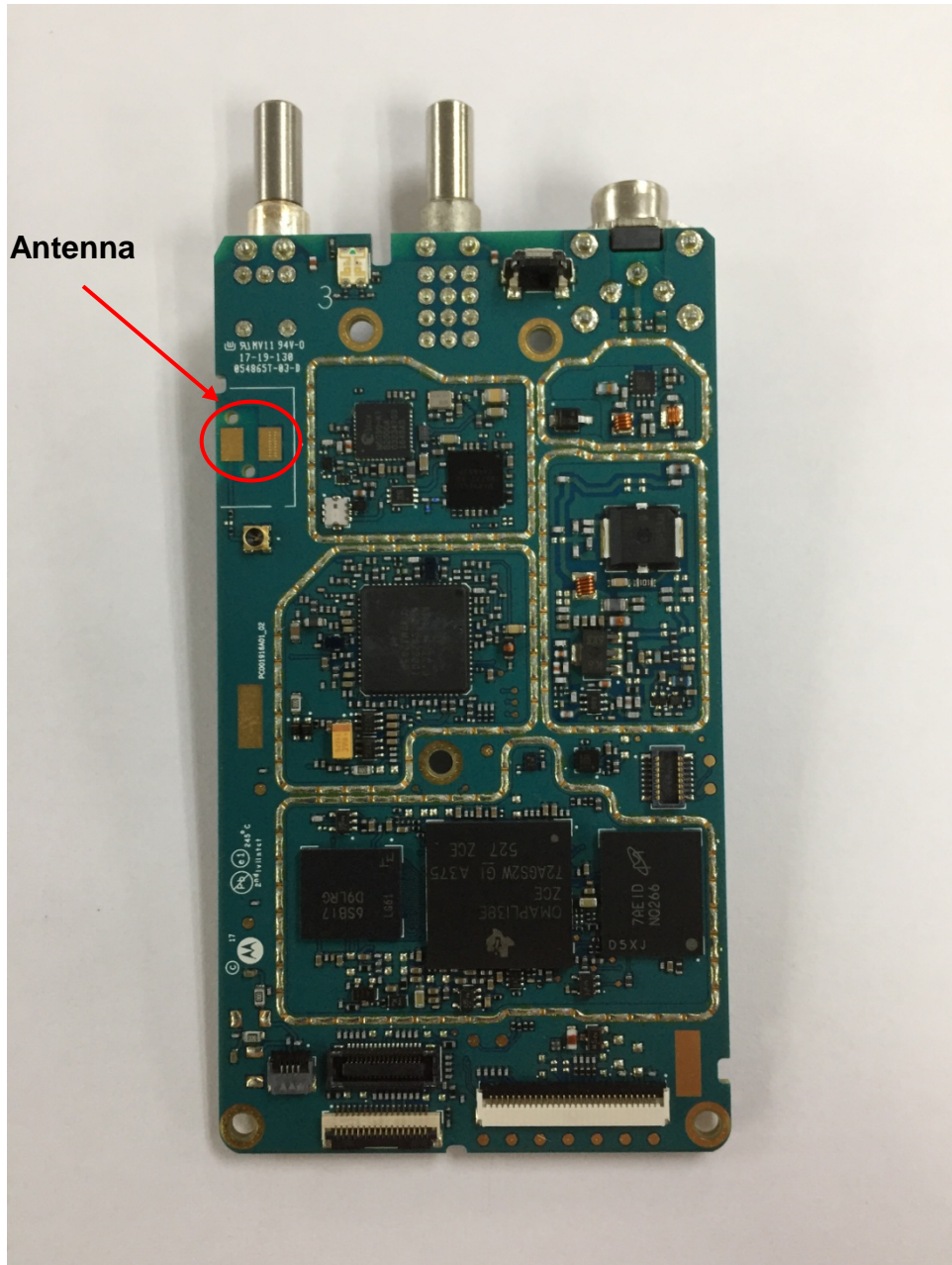
RF board without Shields (Top) (APX900)
