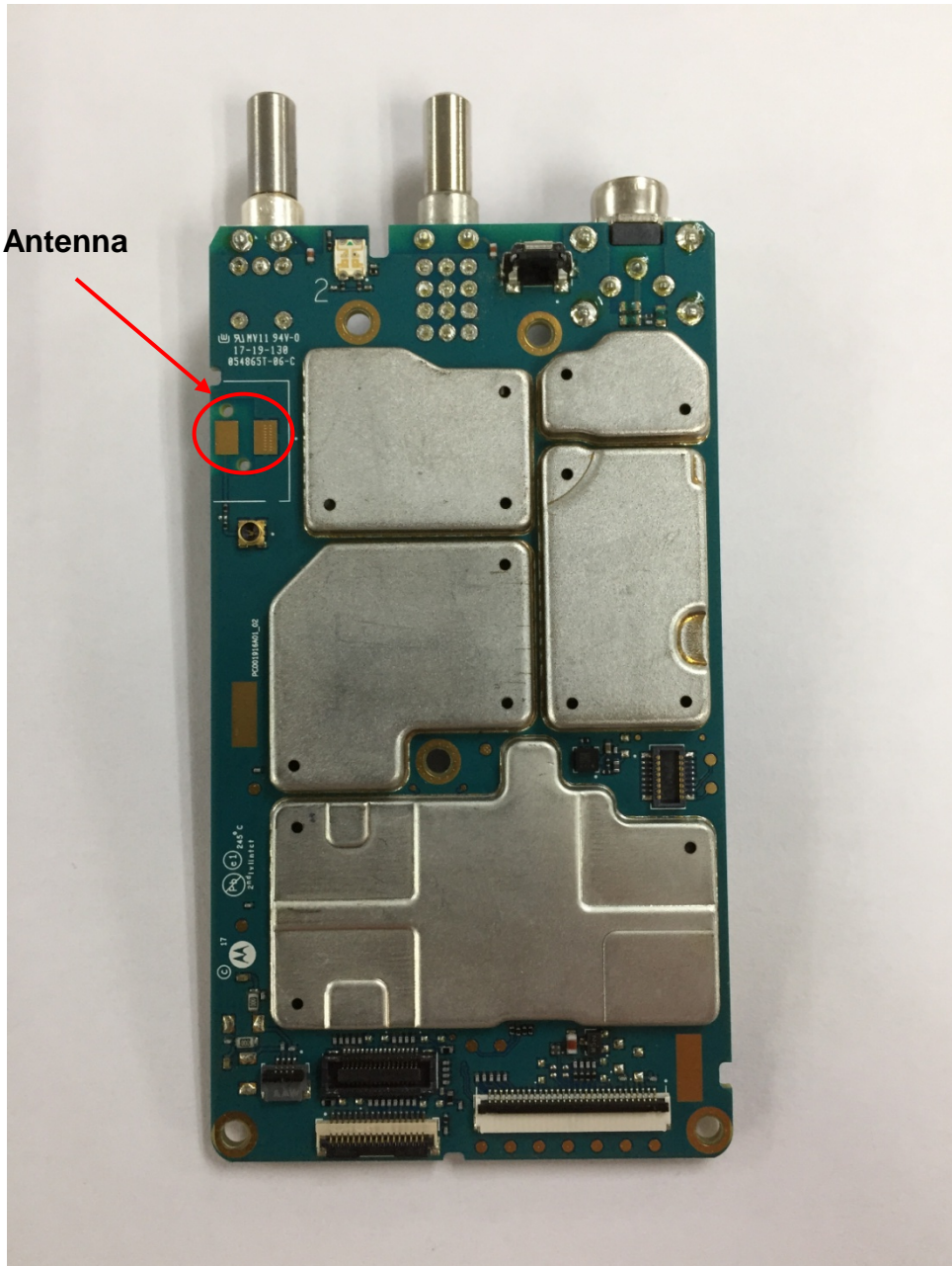
RF board with Shields (Top) (APX900)
