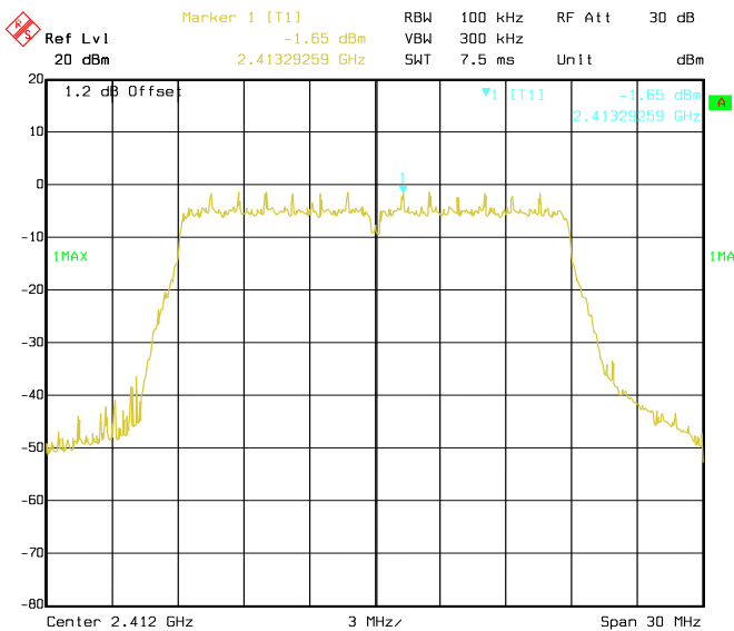
Date: 10.JUL.2017 13:14:07 Conducted Emissions. 802.11n, Frequency 2412 MHz Reference Level
