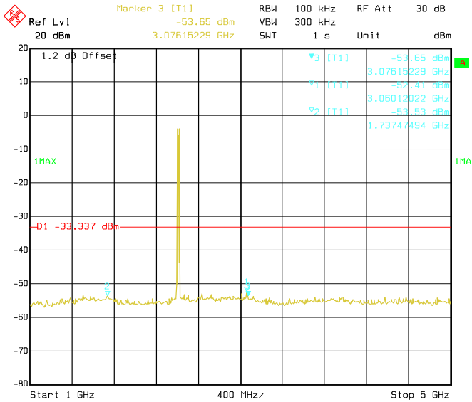
Conducted Emissions. 802.11g, Frequency 2412 MHz Emission Level, 1 GHz -> 5 GHz
