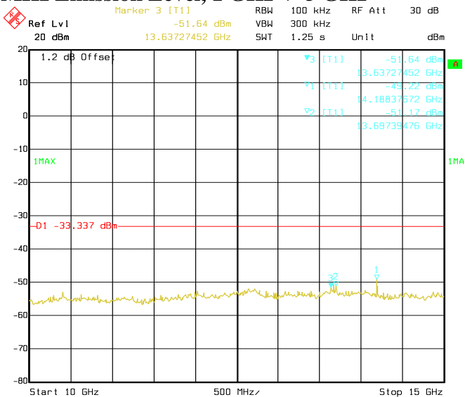
Conducted Emissions. 802.11g, Frequency 2412 MHz Emission Level, 10 GHz -> 15 GHz
