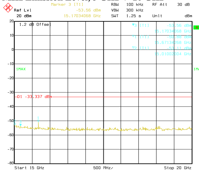
Conducted Emissions. 802.11g, Frequency 2412 MHz Emission Level, 15 GHz -> 20 GHz
