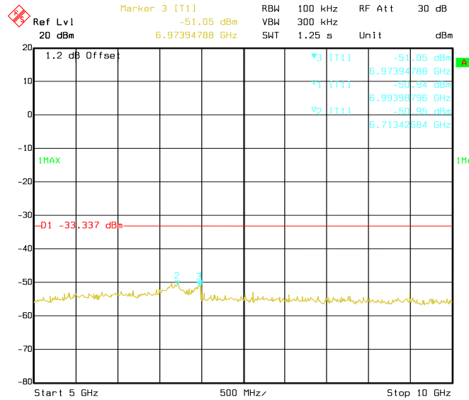
Conducted Emissions. 802.11g, Frequency 2412 MHz Emission Level, 5 GHz -> 10 GHz
