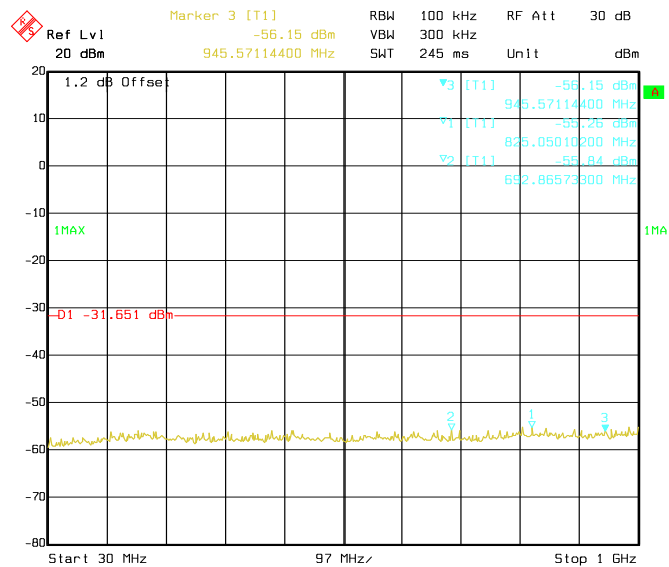
Date: 10.JUL.2017 13:15:02 Conducted Emissions. 802.11n, Frequency 2412 MHz Emission Level, 30 MHz -> 1 GHz
