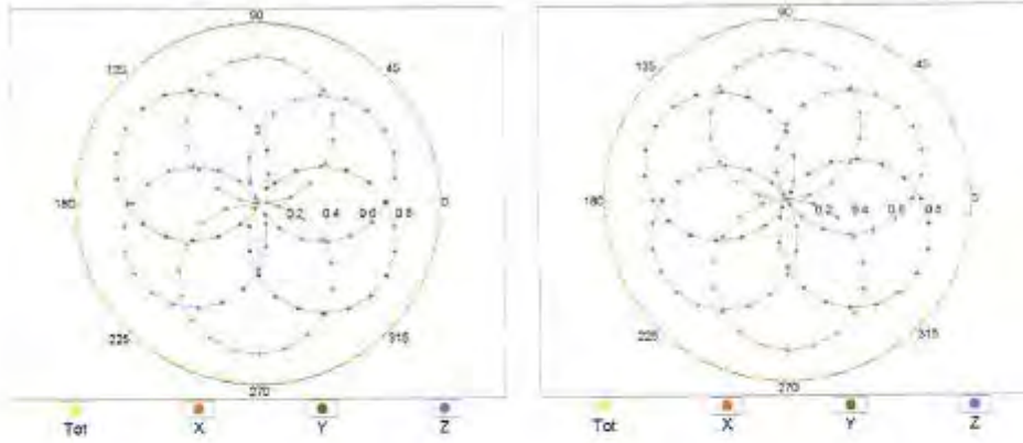
f=600 MHz,TEM
