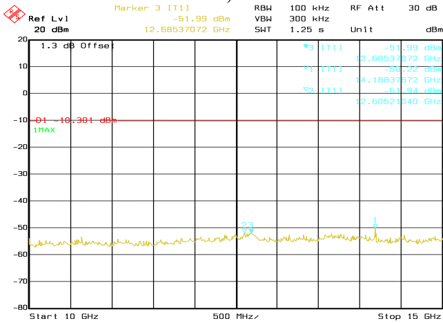
Date: 02.DEC.2016 11:49:14 Conducted Emissions. Bluetooth LE, Frequency 2480 MHz Emission Level, 10 GHz -> 15 GHz
