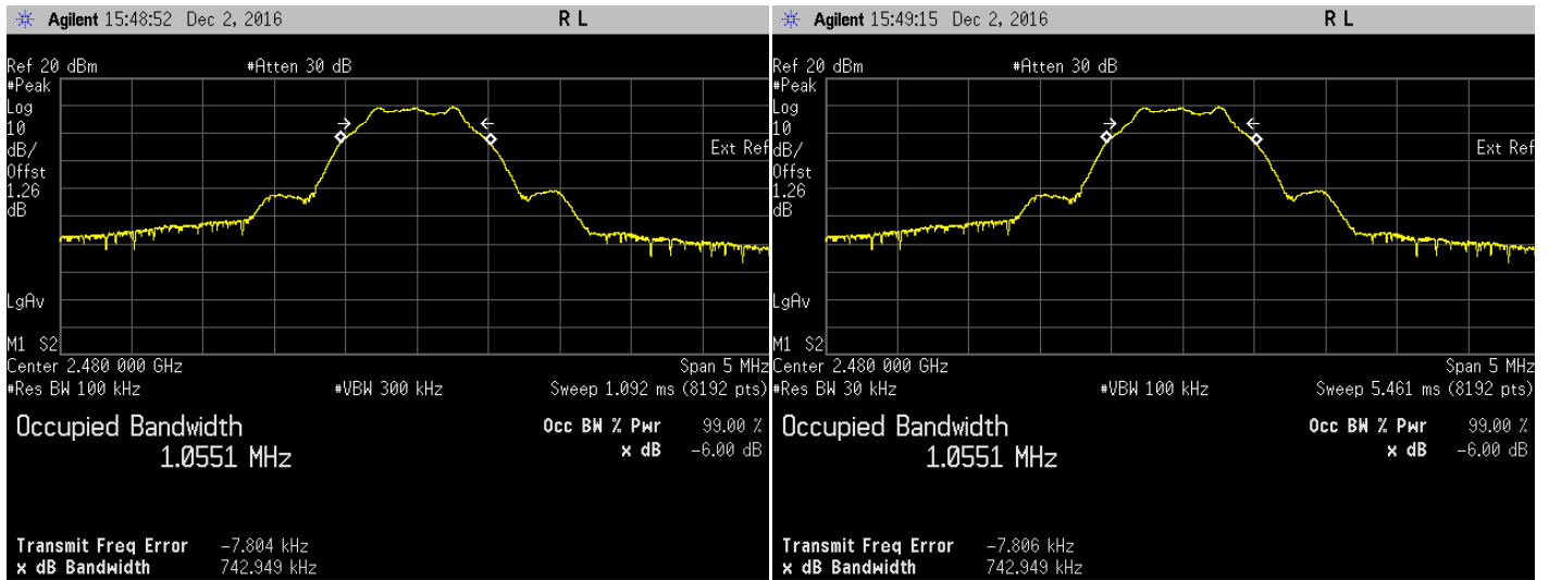
6dB Bandwidth. Bluetooth LE Frequency 2480 MHz
