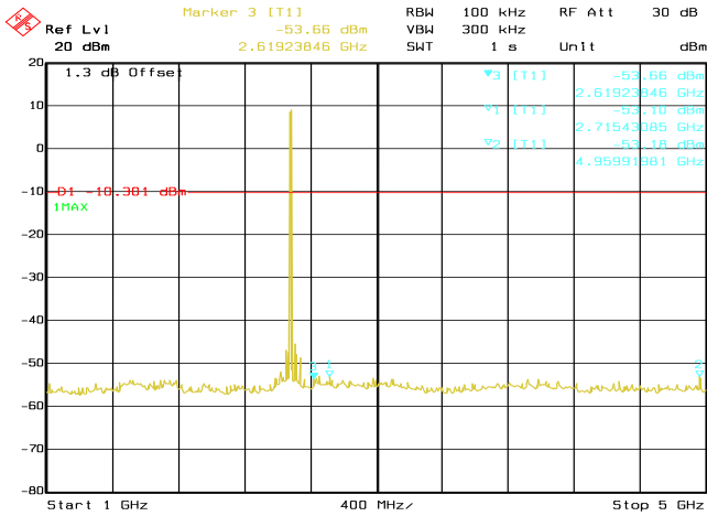
Date: 02.DEC.2016 11:48:08 Conducted Emissions. Bluetooth LE, Frequency 2480 MHz Emission Level, 1 GHz -> 5 GHz
