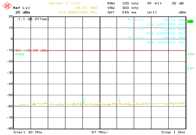
Conducted Emissions. Bluetooth LE, Frequency 2440 MHz Emission Level, 30 MHz -> 1 GHz
