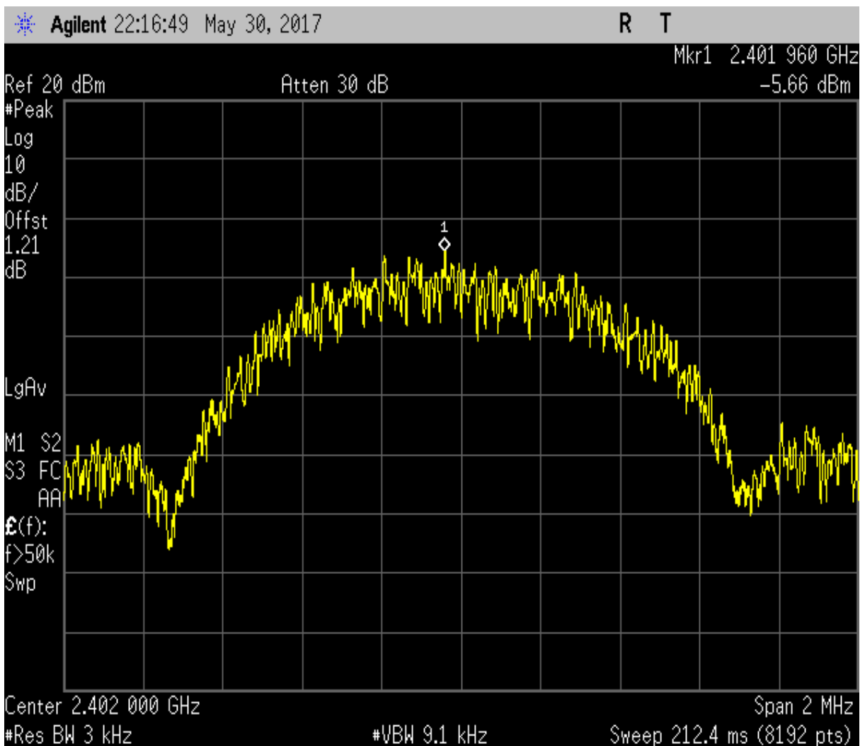
Maximum Power Spectral Density. Bluetooth LE Frequency 2402 MHz
