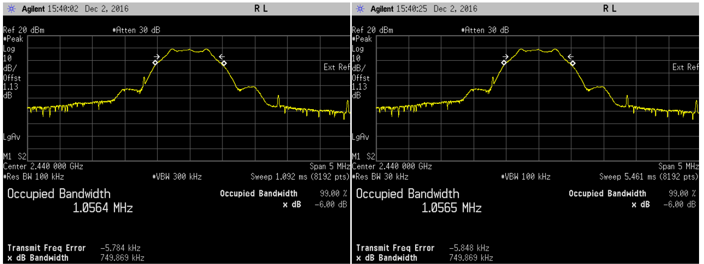
6dB Bandwidth. Bluetooth LE Frequency 2440 MHz
