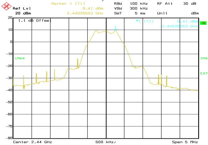
Conducted Emissions. Bluetooth LE, Frequency 2440 MHz Reference Level
