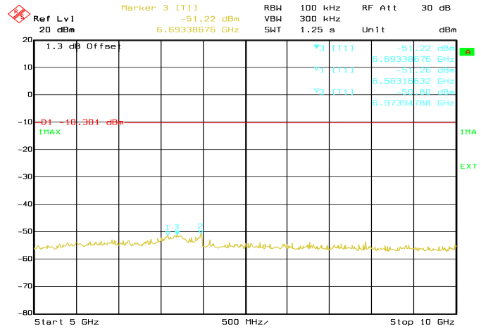
Date: 02.DEC.2016 11:48:41 Conducted Emissions. Bluetooth LE, Frequency 2480 MHz Emission Level, 5 GHz -> 10 GHz
