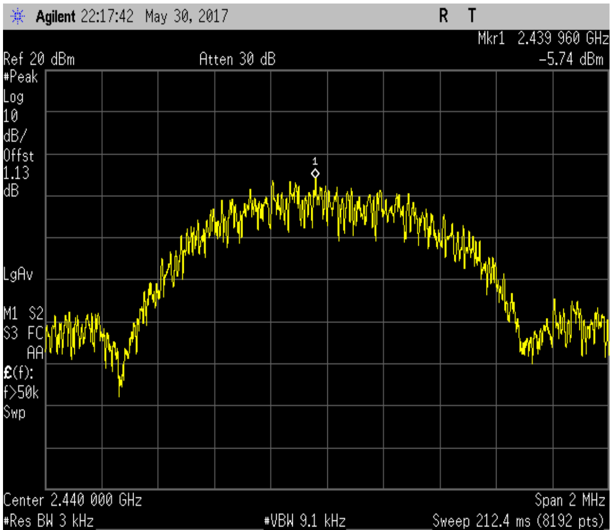
Maximum Power Spectral Density. Bluetooth LE Frequency 2440 MHz
