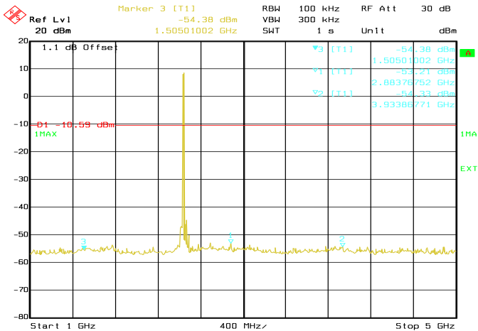
Conducted Emissions. Bluetooth LE, Frequency 2440 MHz Emission Level, 1 GHz -> 5 GHz
