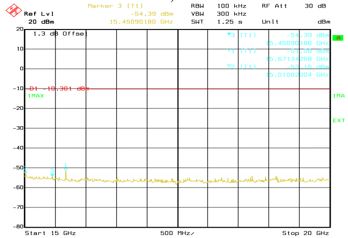
Date: 02.DEC.2016 11:49:46 Conducted Emissions. Bluetooth LE, Frequency 2480 MHz Emission Level, 15 GHz -> 20 GHz
