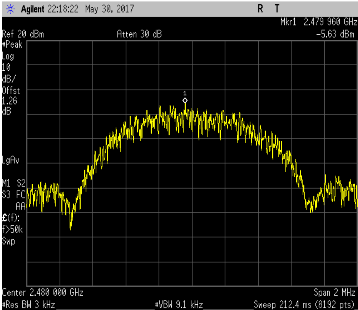
Maximum Power Spectral Density. Bluetooth LE Frequency 2480 MHz
