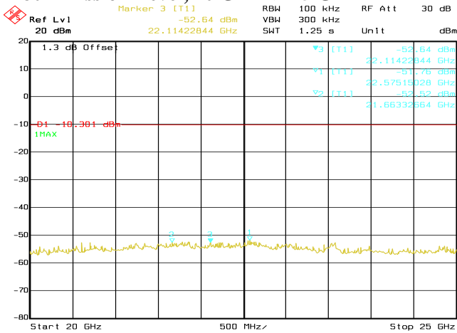
Date: 02.DEC.2016 11:50:20 Conducted Emissions. Bluetooth LE, Frequency 2480 MHz Emission Level, 20 GHz -> 25 GHz
