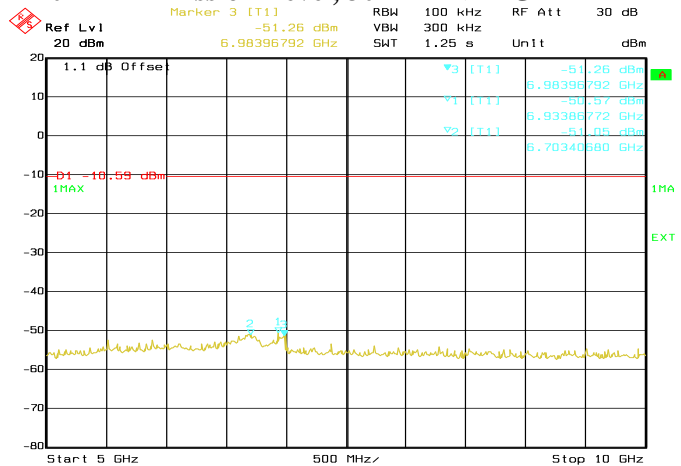
Conducted Emissions. Bluetooth LE, Frequency 2440 MHz Emission Level, 5 GHz -> 10 GHz
