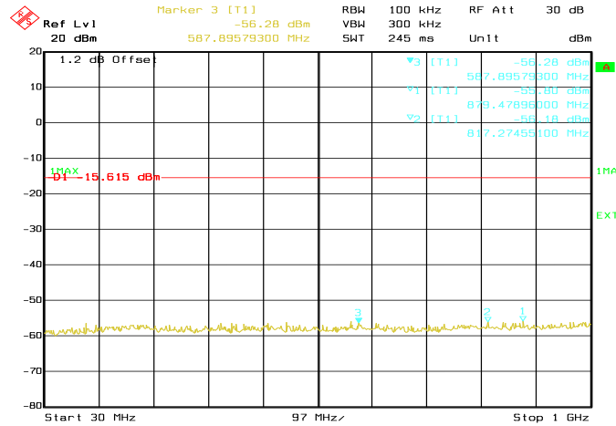
Conducted Emissions. 802.11b, Frequency 2412 MHz Emission Level, 30 MHz -> 1 GHz
