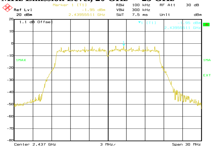
Conducted Emissions. 802.11g, Frequency 2437 MHz Reference Level
