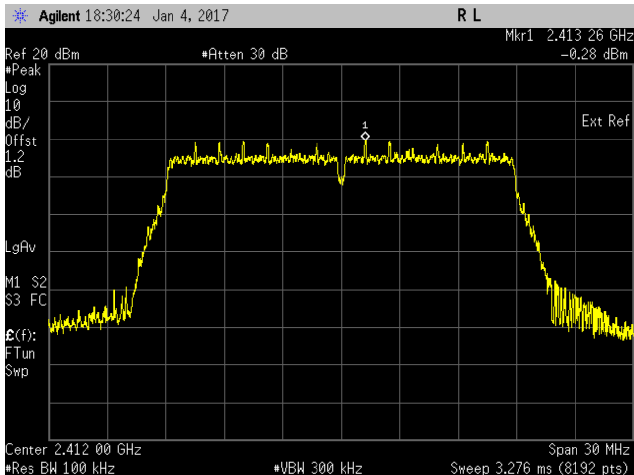
Band Edge. 802.11n Frequency 2412 MHz Reference Level
