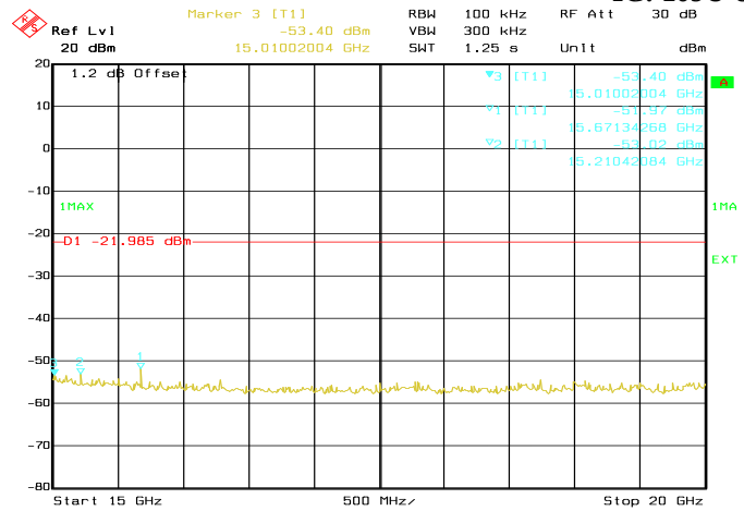
Conducted Emissions. 802.11g, Frequency 2412 MHz Emission Level, 15 GHz -> 20 GHz
