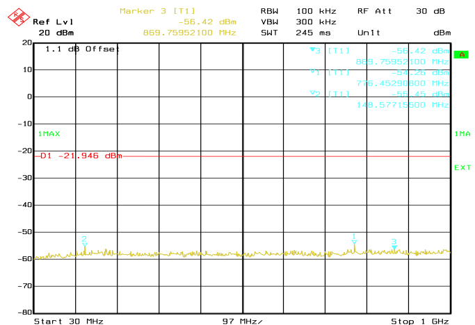
Conducted Emissions. 802.11g, Frequency 2437 MHz Emission Level, 30 MHz -> 1 GHz
