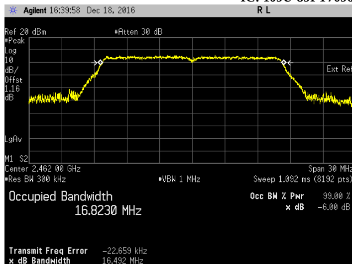
99% Bandwidth. 802.11g Frequency 2462 MHz
