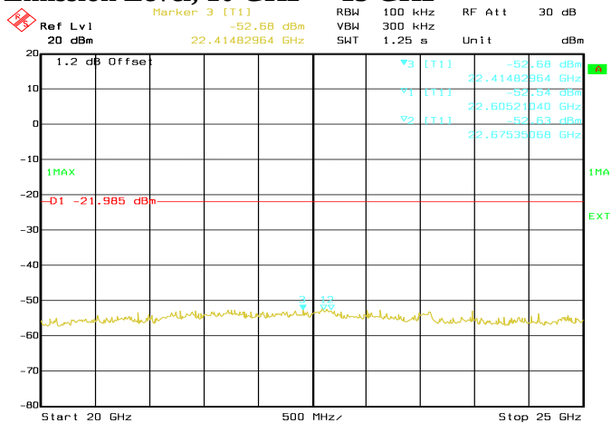
Conducted Emissions. 802.11g, Frequency 2412 MHz Emission Level, 20 GHz -> 25 GHz
