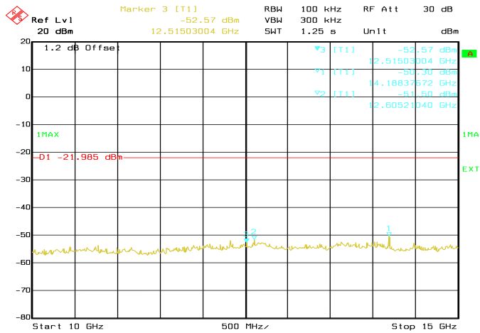
Conducted Emissions. 802.11g, Frequency 2412 MHz Emission Level, 10 GHz -> 15 GHz
