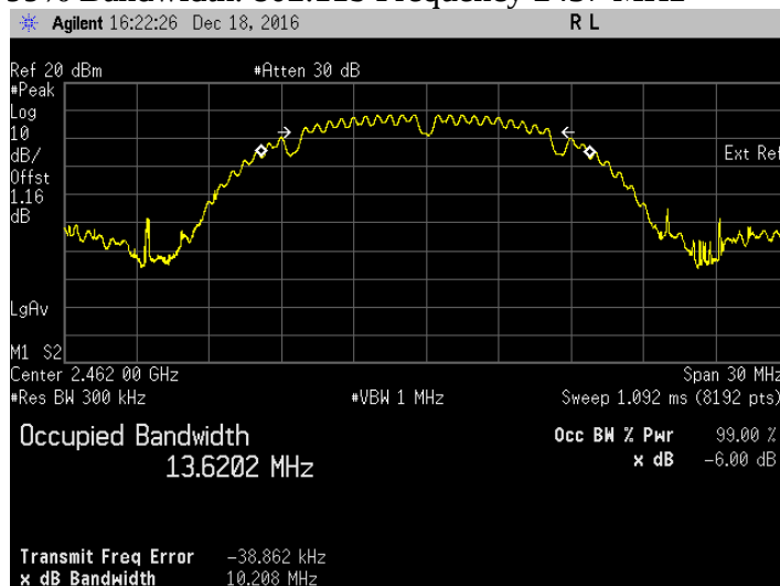
99% Bandwidth. 802.11b Frequency 2462 MHz
